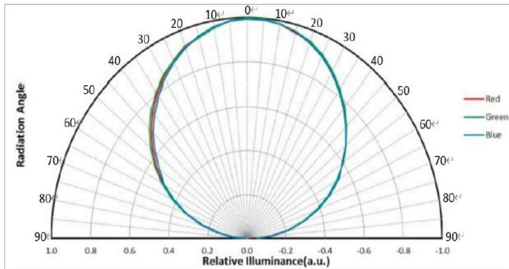
Radiation Diagram
