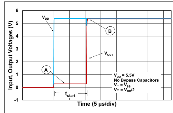
FIGURE 4-13: Start-up Test Waveforms.
