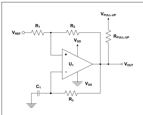
FIGURE 4-17: Bistable Multivibrator.
