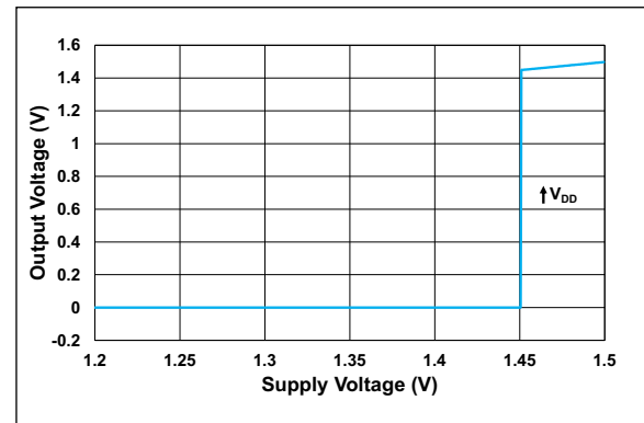
FIGURE 4-5: POR Rising.
