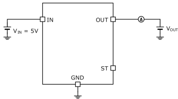
Measurement Circuit for Figure 18, Figure 19
