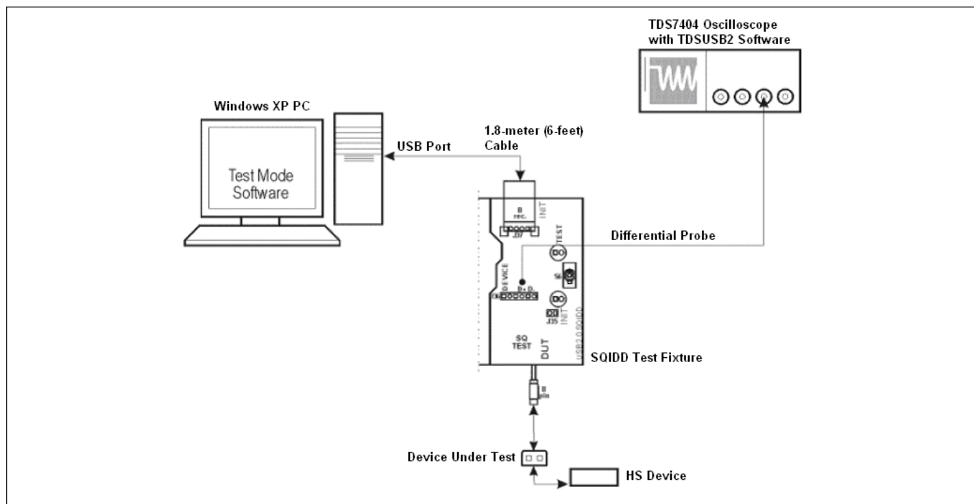
Figure 1: HS Eye Test Setup
