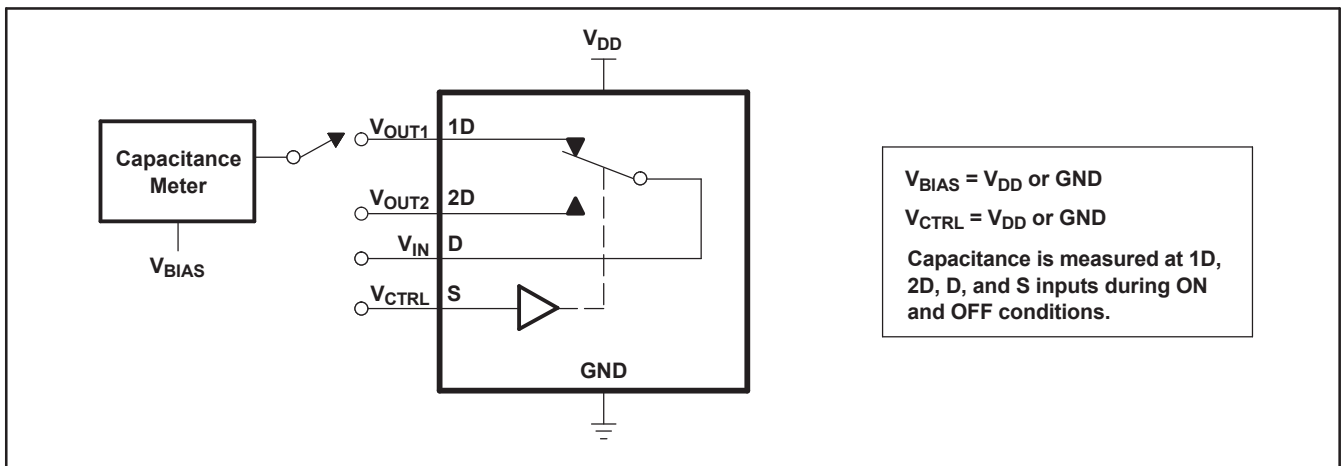
Figure 10. Capacitance
