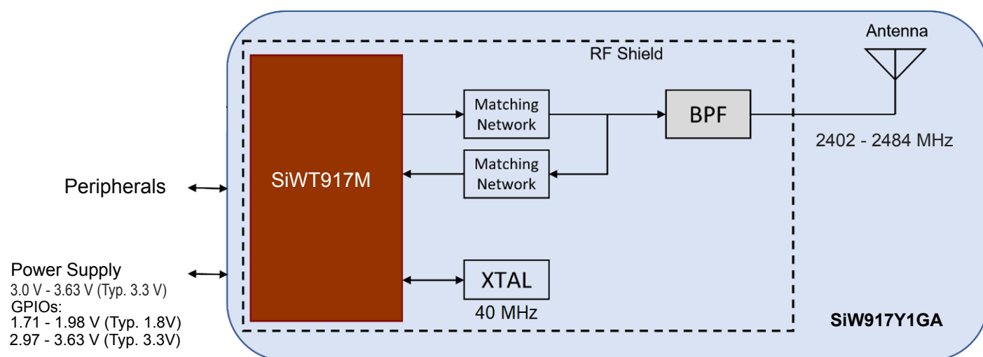
Figure 4.2. SiW917Y1GA (With Antenna) Module Block Diagram
