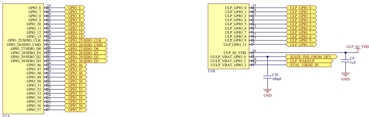
Figure 8.3. GPIO Connection
