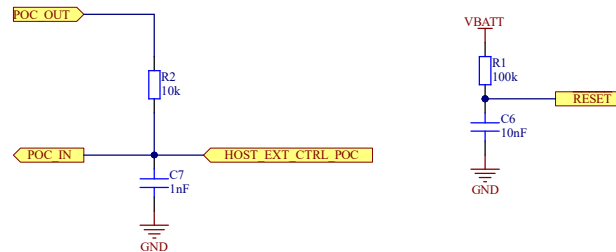
Figure 8.10. Reset Configuration
