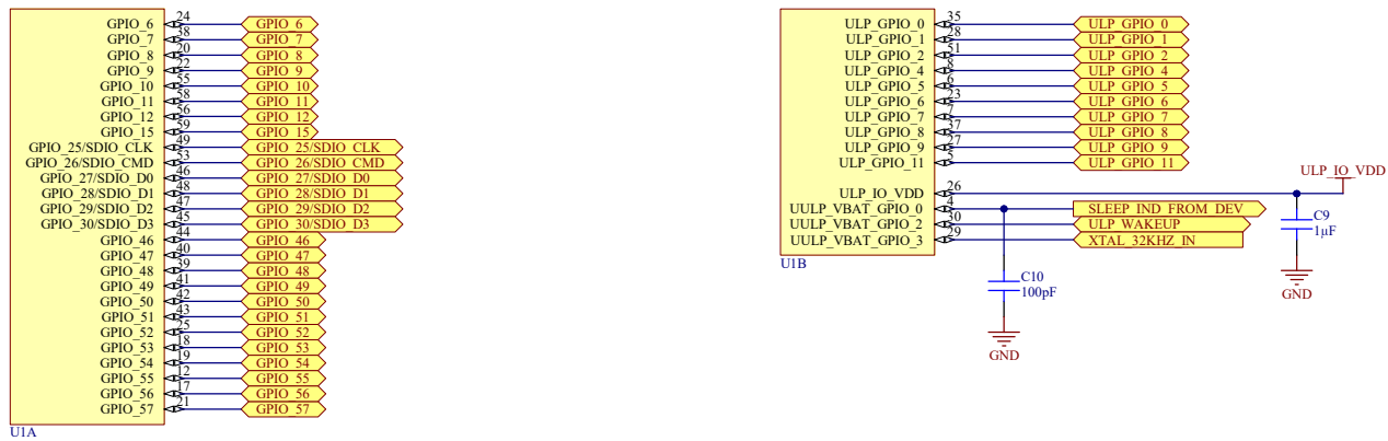
Figure 8.9. GPIO Connection
