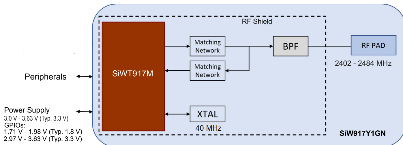
Figure 4.1. SiW917Y1GN (Without Antenna) Module Block Diagram
