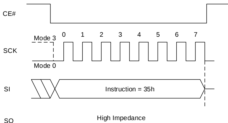
Figure 8.54 Enter Quad Peripheral Interface (QPI) Mode Sequence
