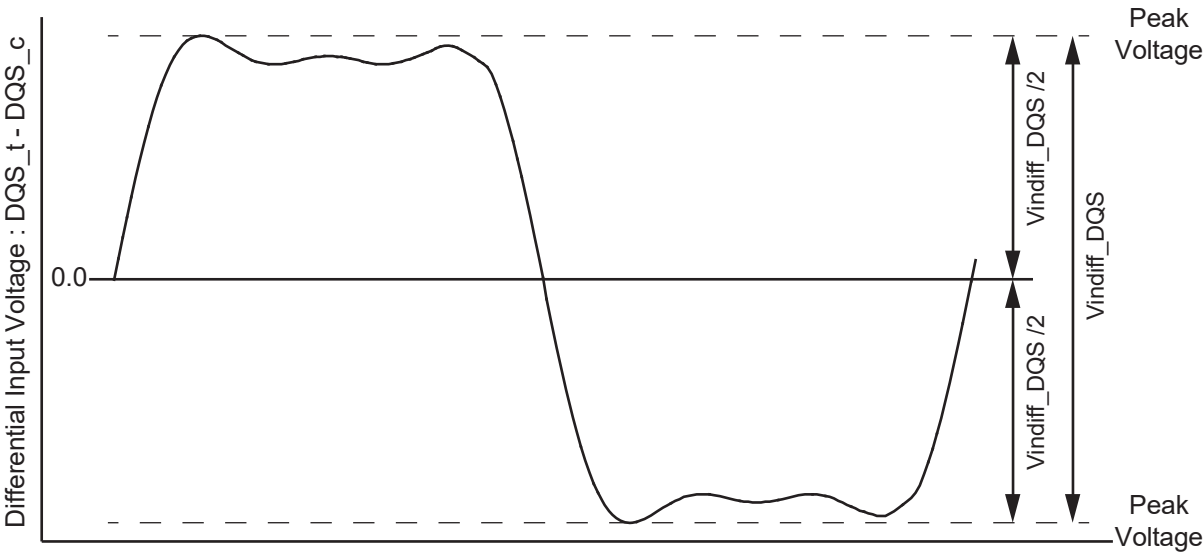
Figure 7.9 — DQS Differential Input Voltage
