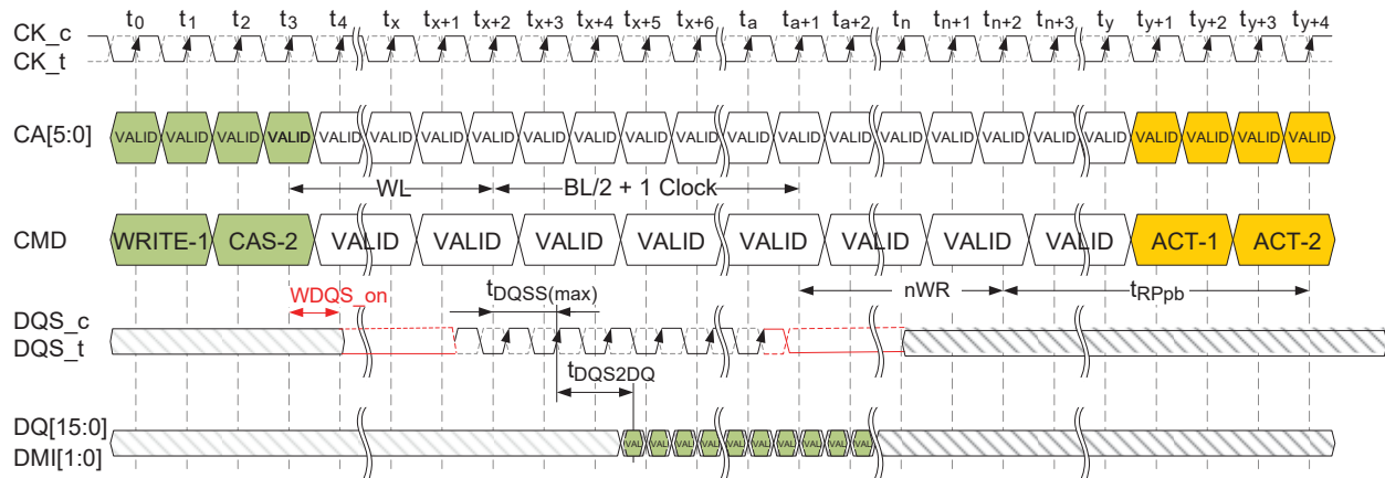
Figure 4.51 — Burst WRITE with Auto-PRECHARGE (Shown with BL16, 2tCK pre-ample)
