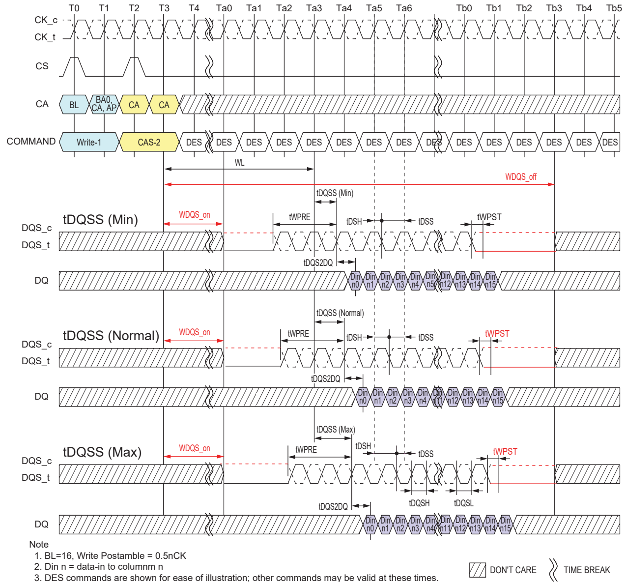
Figure 4.16 — Write Timing
