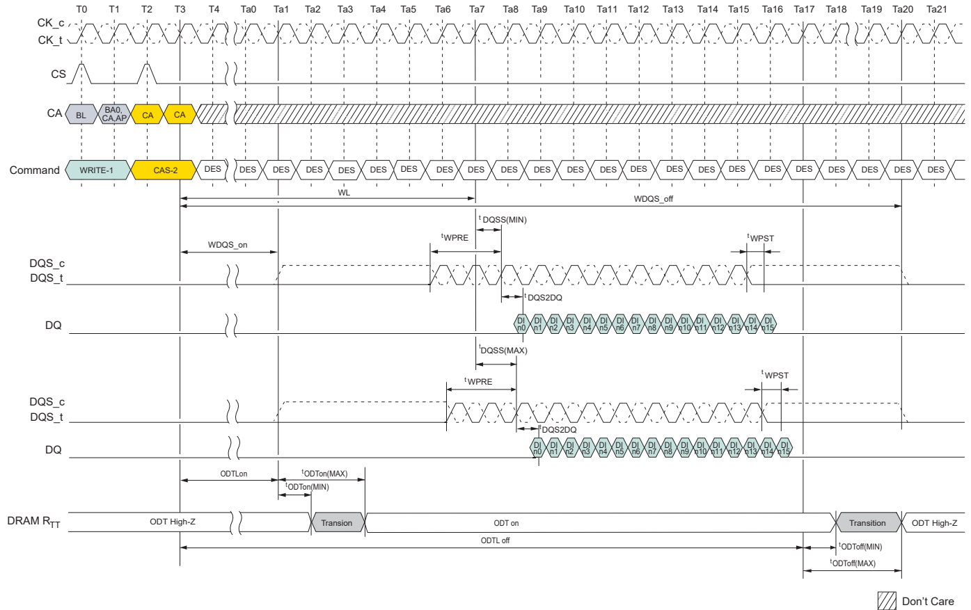
Figure 4.132: Burst WRITE Operation
