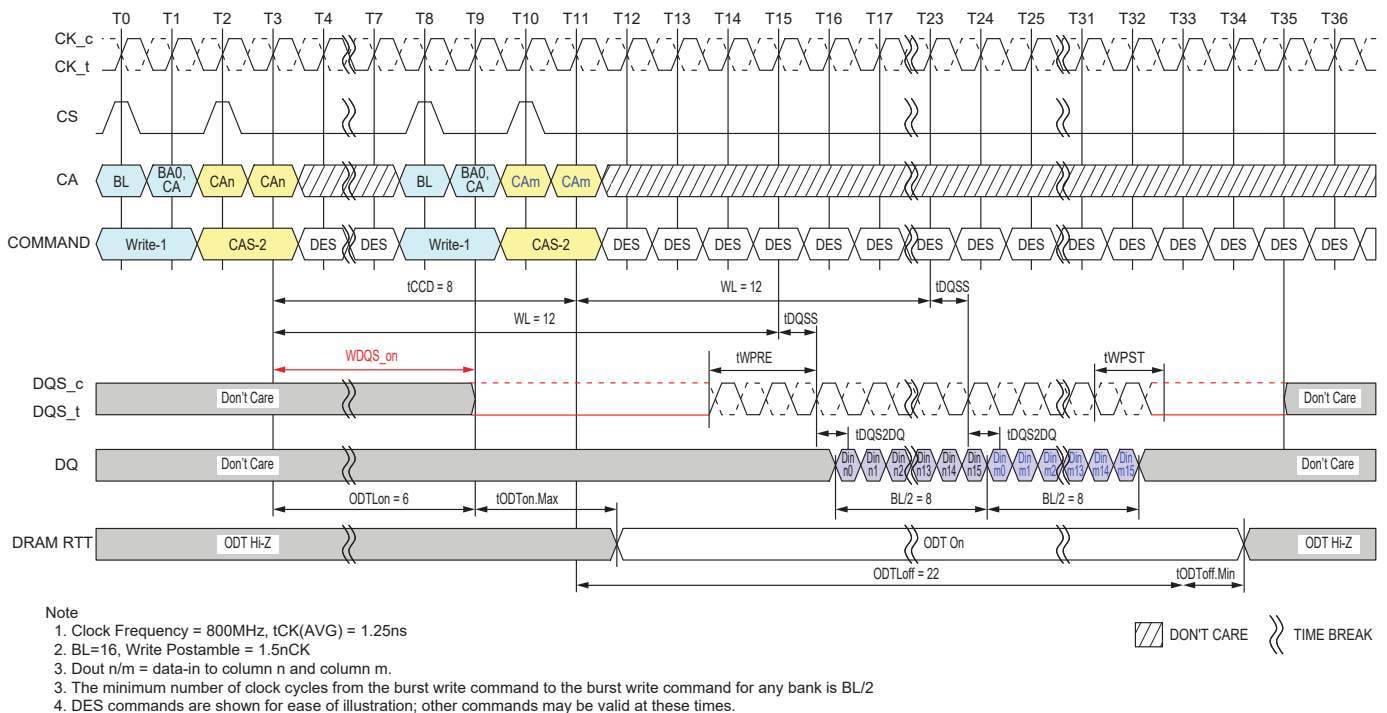
Figure 4.33 — Seamless Writes Operation: tCCD = Min, 1.5nCK Postamble, 533MHz &lt; Clock Freq. ≤ 800MHz, ODT Worst Timing Case
