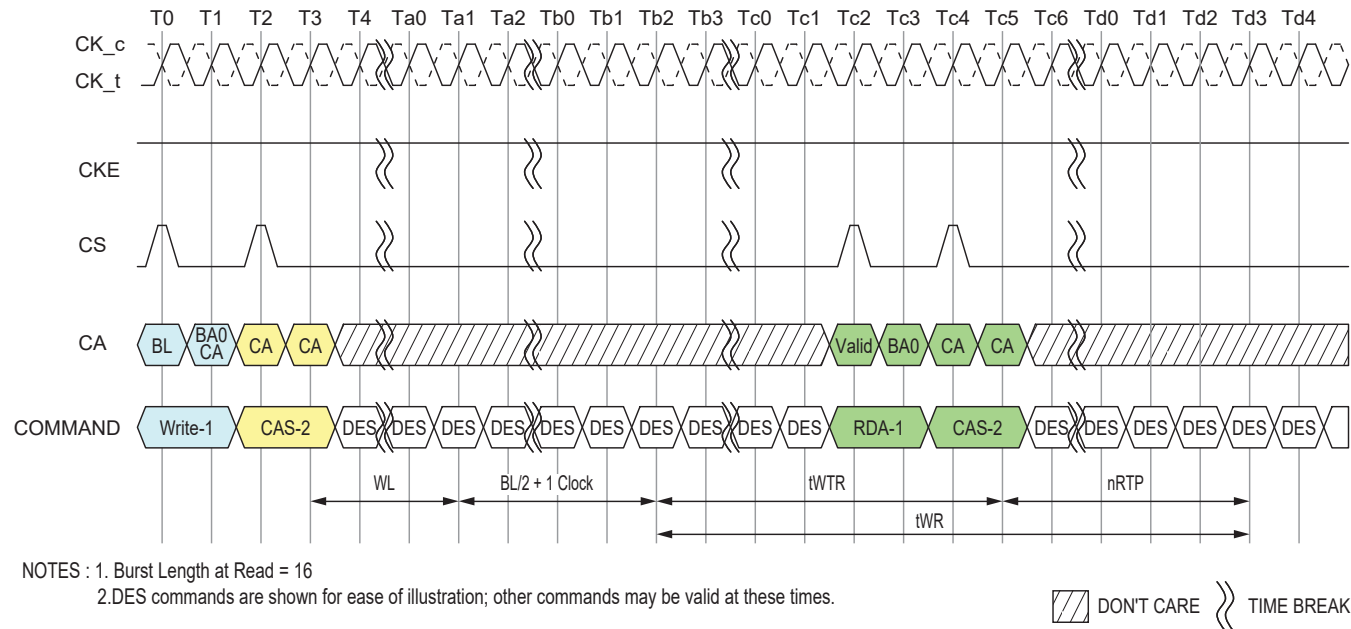
Figure 4.53 — Delay time from Write to Read with Auto-Precharge
