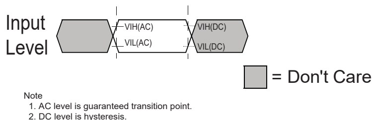
Figure 7.1 — Input Timing Definition for CKE
