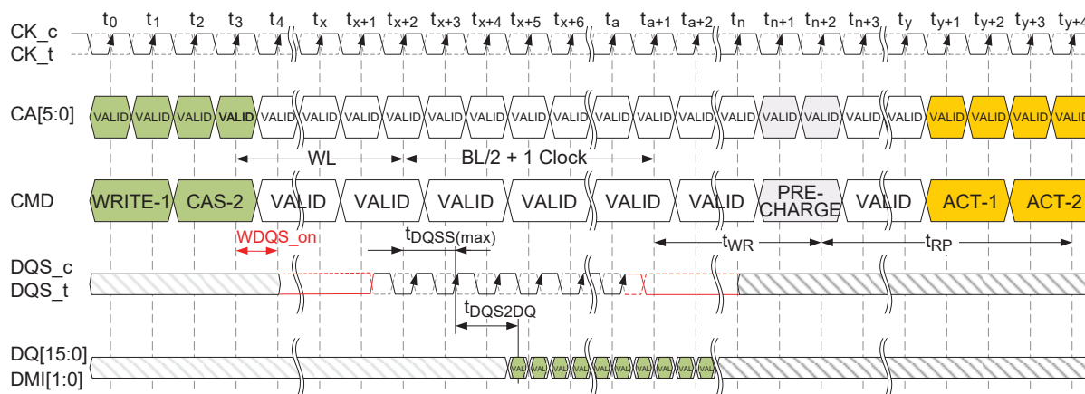
Figure 4.48— Burst WRITE Followed by PRECHARGE (Shown with BL16, 2tCK pre-ample)
