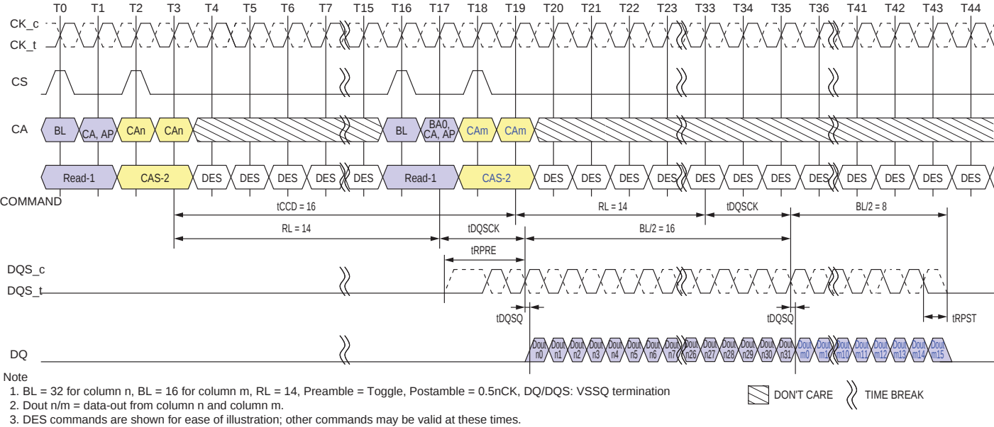
Figure 4.4 — Burst Read Timing
