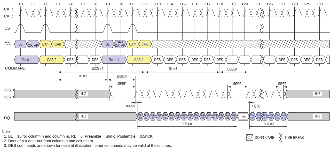
Figure 4.23 — Consecutive Reads Operation: tCCD = Min +1, Preamble = Static, 0.5nCK Postamble
