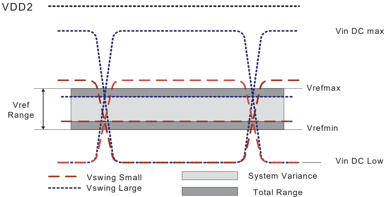
Figure 4.69 — V REF operating range(V REF min, V REF max)
