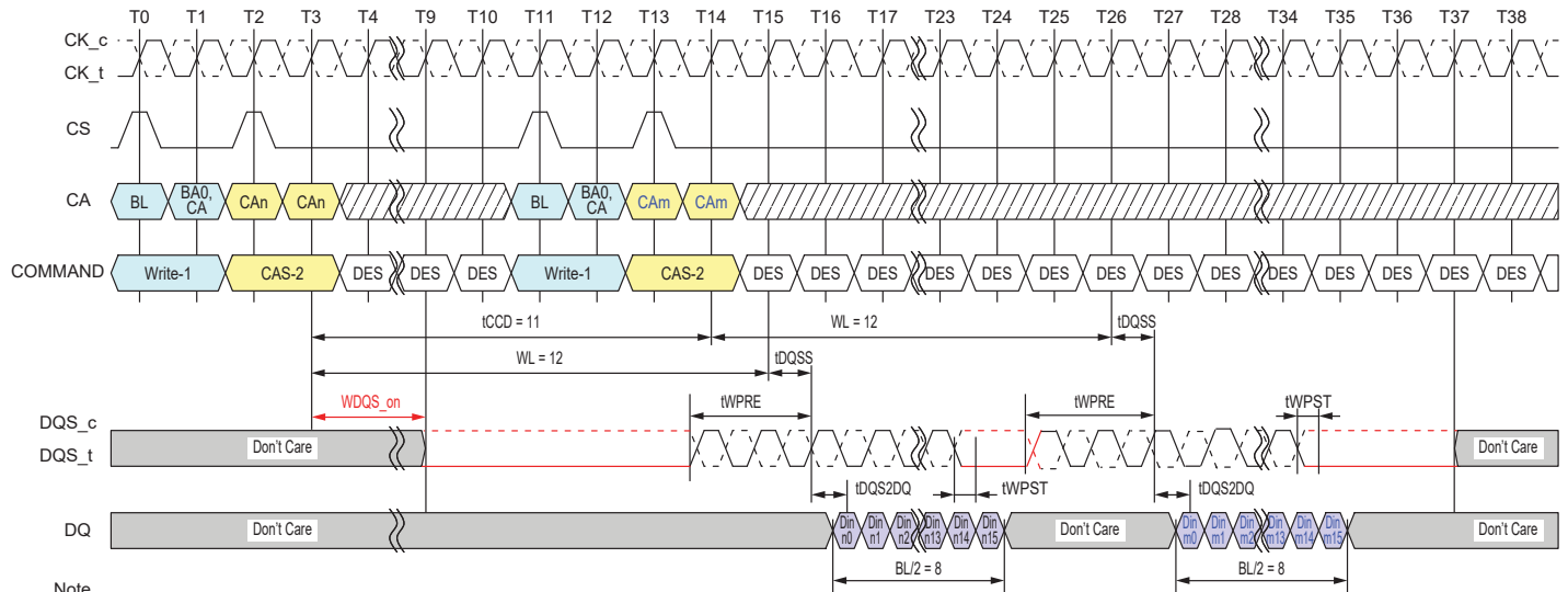
Figure 4.39 — Consecutive Writes Operation: t_{CCD} = \text{Min} + 3, 0.5n\text{CK} Postamble
