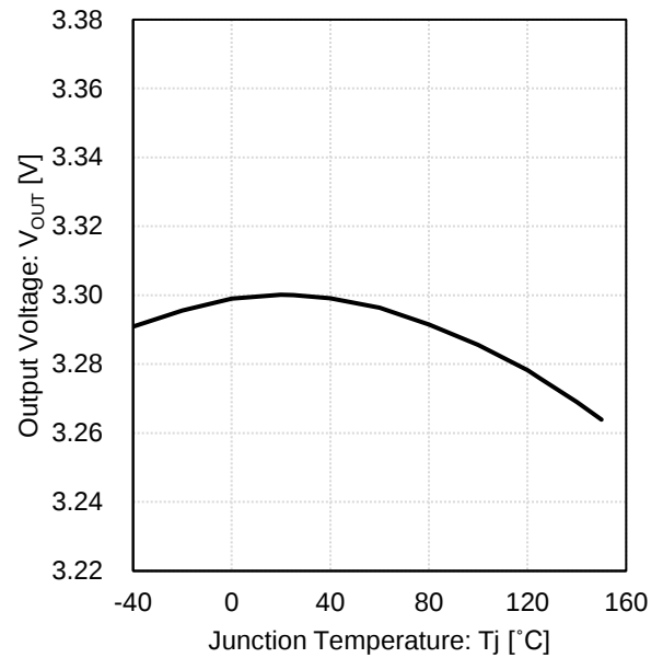
Figure 36. Output Voltage vs Junction Temperature (3.3 V output)
