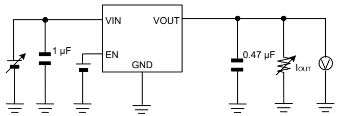
Measurement Setup for Figure 6, 9 to 12, 14, 36, 39 to 41
