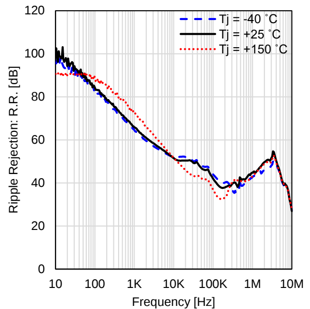
Figure 38. Ripple Rejection vs Frequency (3.3 V output, V_{Ripple} = 1\text{ Vrms} , I_{OUT} = 10\text{ mA} )
