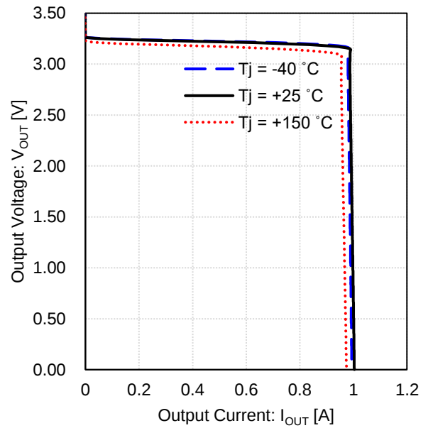
Figure 42. Output Voltage vs Output Current (3.3 V output, Over Current Protection)
