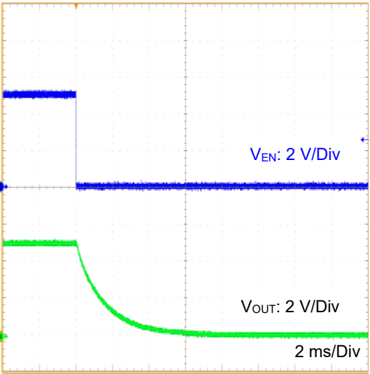
Figure 30. EN Shutdown Waveform (5 V output, I_{OUT} = 1\text{ mA} )
