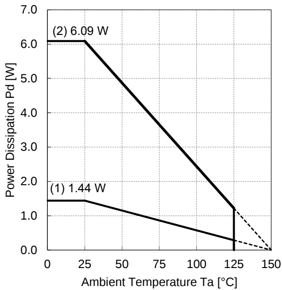
Figure 68. Power Dissipation Graph (TO263-3 / TO263-5)
