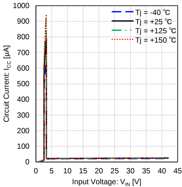
Figure 31. Circuit Current vs Input Voltage (3.3 V output)
