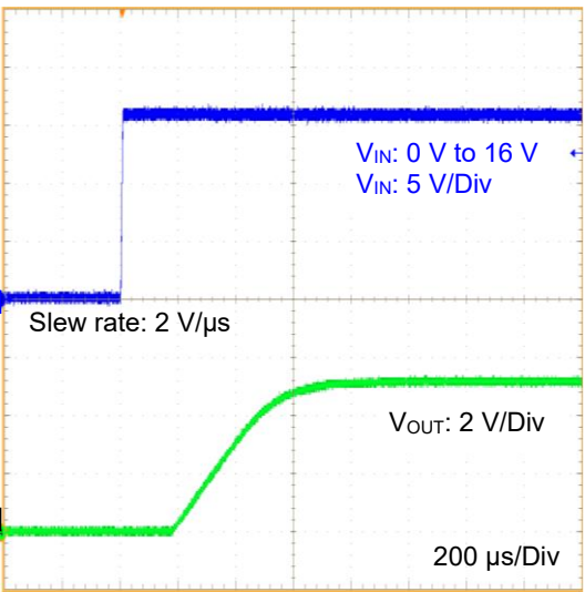
Figure 28. VIN Startup Waveform V_{IN} : 0 V to 16 V (5 V output, I_{OUT} = 500\text{ mA} )
