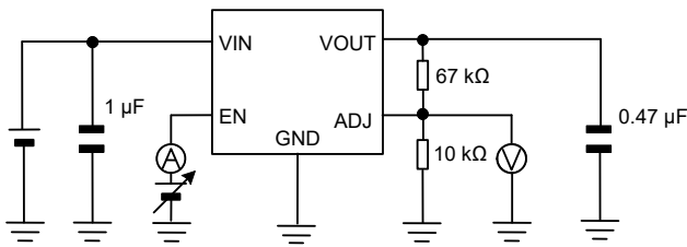
Measurement Setup for Figure 15
