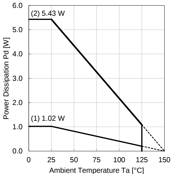
Figure 67. Power Dissipation Graph (TO252-3 / TO252-5)
