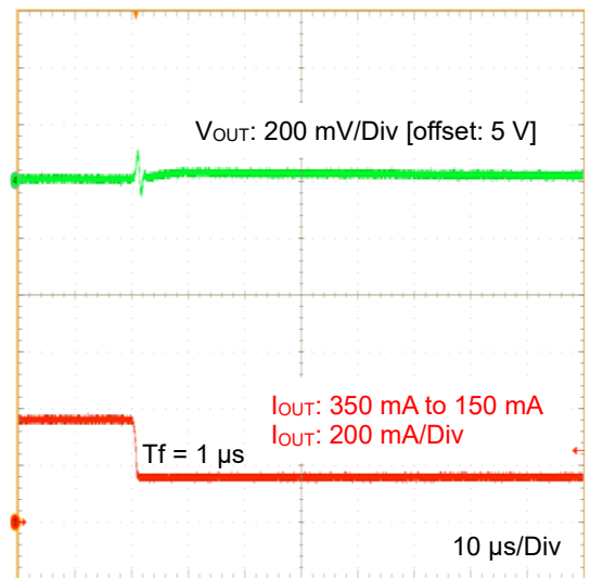
Figure 22. Load Transient 350 mA to 150 mA (5 V output, T_f = 1\text{ }\mu\text{s} )
