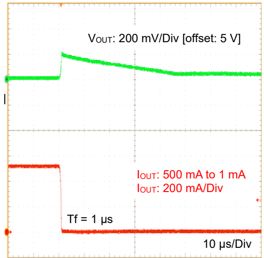
Figure 20. Load Transient 500 mA to 1 mA (5 V output, T_f = 1\text{ }\mu\text{s} )
