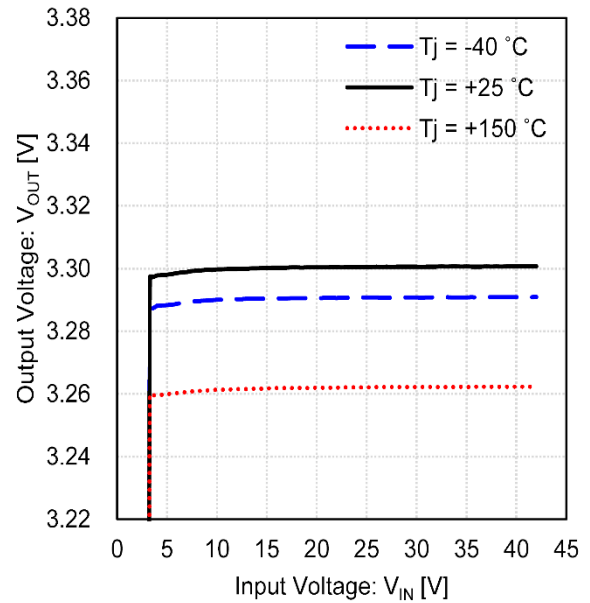
Figure 40. Output Voltage vs Input Voltage; Enlarged view of Figure 39 at narrow Output Voltage range (3.3 V output)
