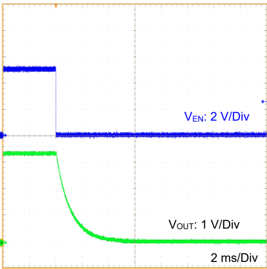
Figure 54. EN Shutdown Waveform (3.3 V output, I_{OUT} = 1\text{ mA} )
