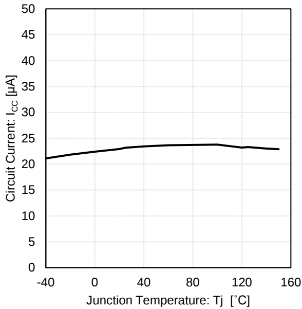
Figure 35. Circuit Current vs Junction Temperature (3.3 V output)
