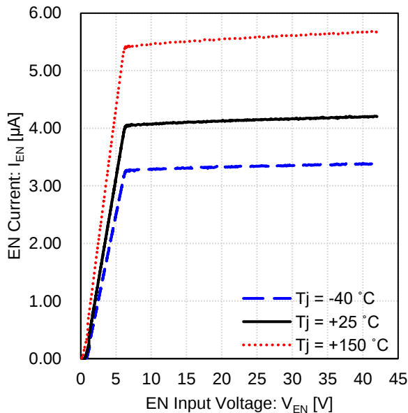
Figure 17. EN Bias Current vs EN Input Voltage
