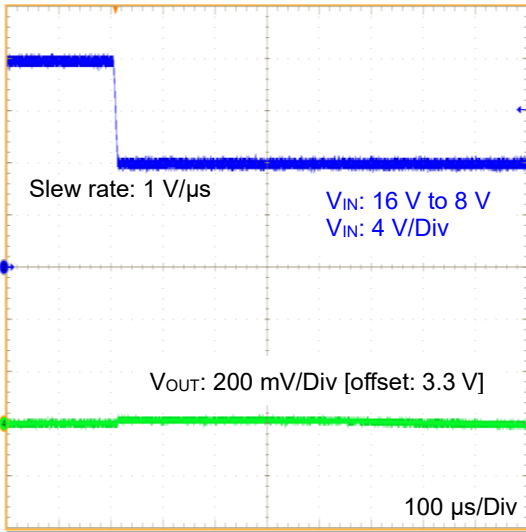
Figure 48. Line Transient 16 V to 8 V (3.3 V output, I_{OUT} = 0\text{ mA} )
