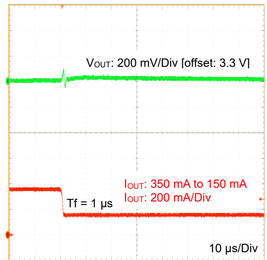
Figure 46. Load Transient 350 mA to 150 mA (3.3 V output, T_f = 1\text{ }\mu\text{s} )
