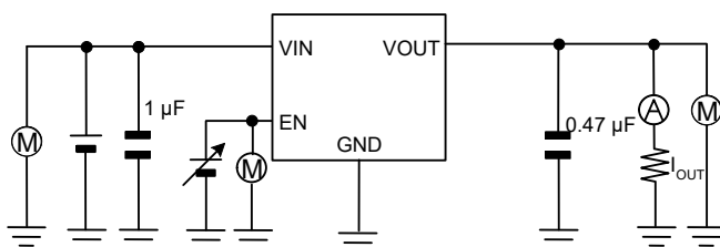
Measurement Setup for Figure 29 to 30, 53 to 54
