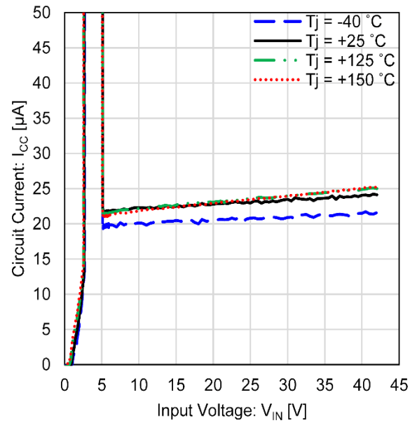
Figure 2. Circuit Current vs Input Voltage; Enlarged view of Figure 1 at narrow Circuit Current range (5 V output)
