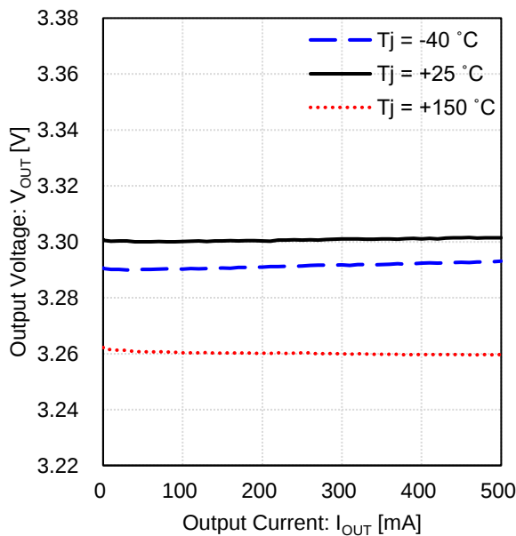
Figure 41. Output Voltage vs Output Current (3.3 V output, Load Regulation)
