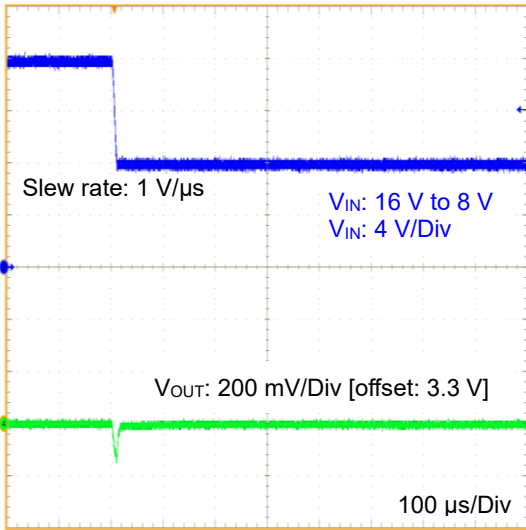
Figure 50. Line Transient 16 V to 8 V (3.3 V output, I_{OUT} = 500\text{ mA} )
