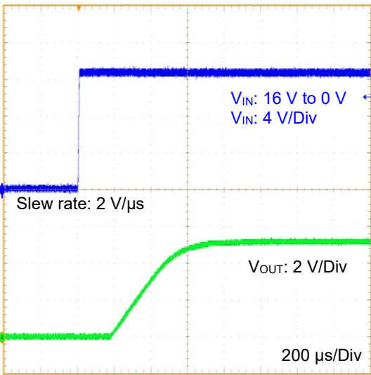
Figure 52. VIN Startup Waveform V_{IN} : 0 V to 16 V (3.3 V output, I_{OUT} = 500\text{ mA} )
