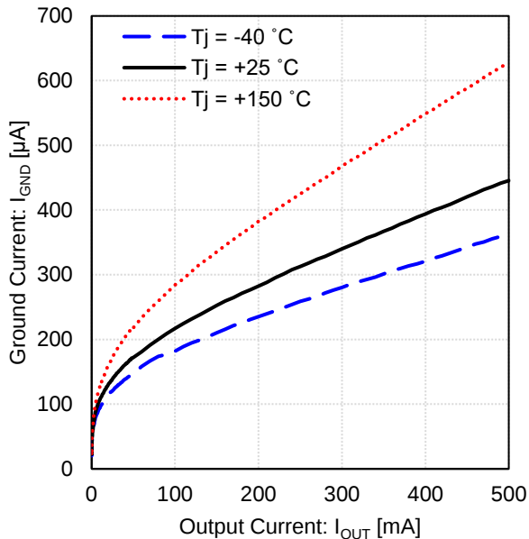
Figure 33. Ground Current vs Output Current (3.3 V output)
