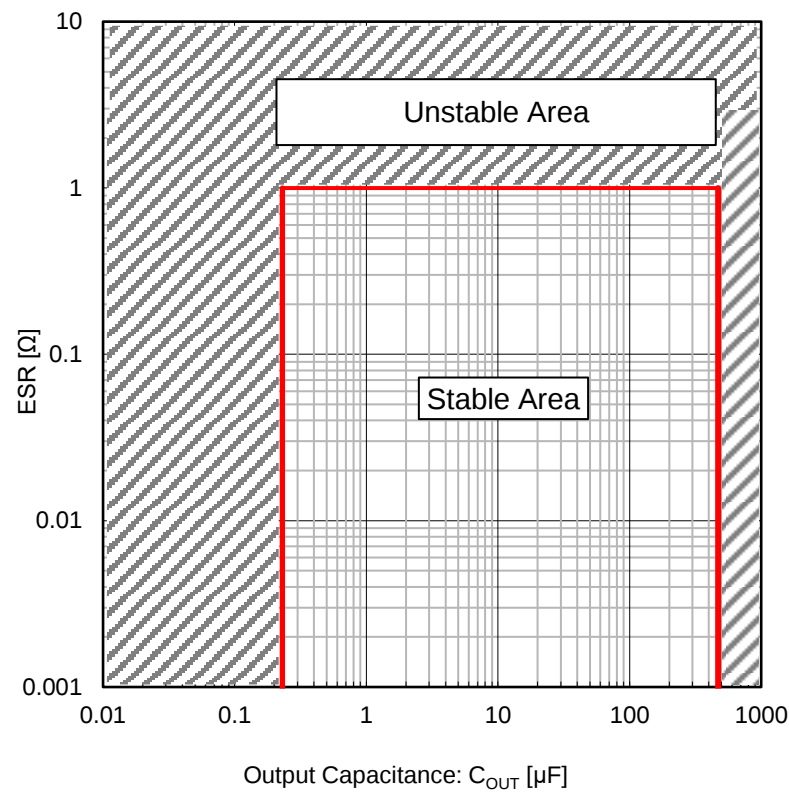
Figure 55. Output Capacitance C_{OUT} , ESR Available Area ( V_{IN} = 4.5\text{ V} to 42\text{ V} , V_{OUT} = 1\text{ V} (Note 1), -40\text{ }^{\circ}\text{C} \leq T_J \leq +150\text{ }^{\circ}\text{C} , I_{OUT} = 0\text{ mA} to 500\text{ mA} ) (Note 1) The most strict condition from the stability theory for the control loop of regulator.
