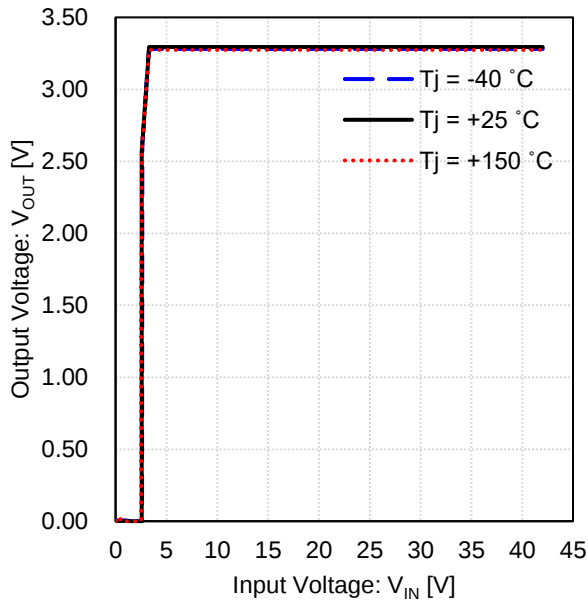
Figure 39. Output Voltage vs Input Voltage (3.3 V output)
