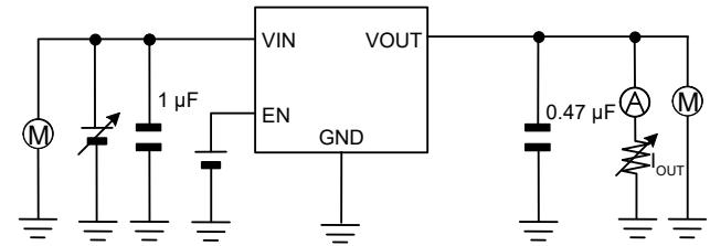
Measurement Setup for Figure 19 to 28, 43 to 52
