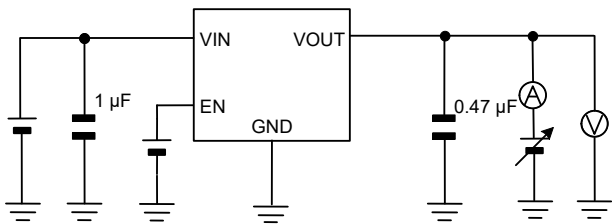
Measurement Setup for Figure 13, 42
