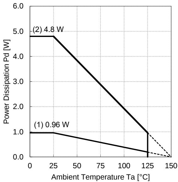
Figure 66. Power Dissipation Graph (HTSOP-J8)
