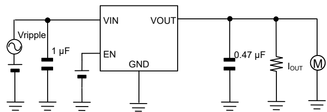
Measurement Setup for Figure 8, 38
