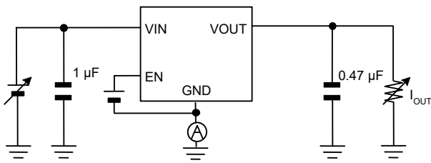
Measurement Setup for Figure 1 to 5, 16, 31 to 35
