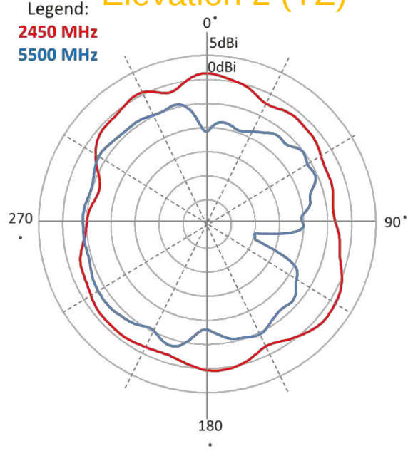
Elevation 2 (YZ)
