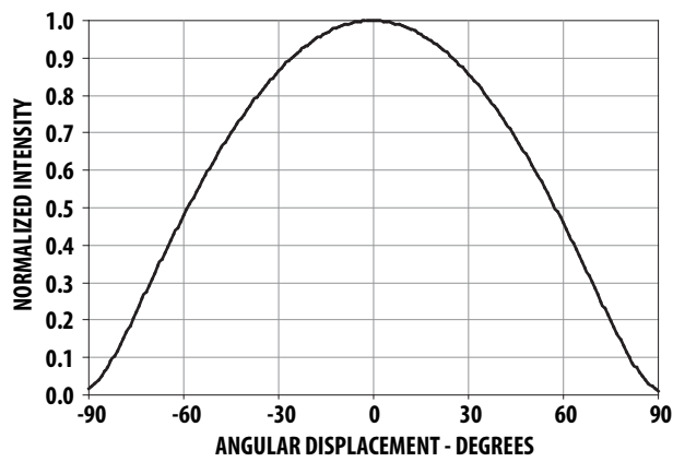
Figure 11. Radiation Pattern
