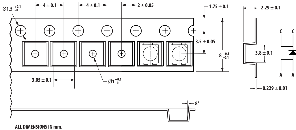
Figure 16. Tape Dimensions
