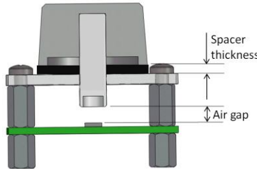
Figure 15: Air Gap Setting
