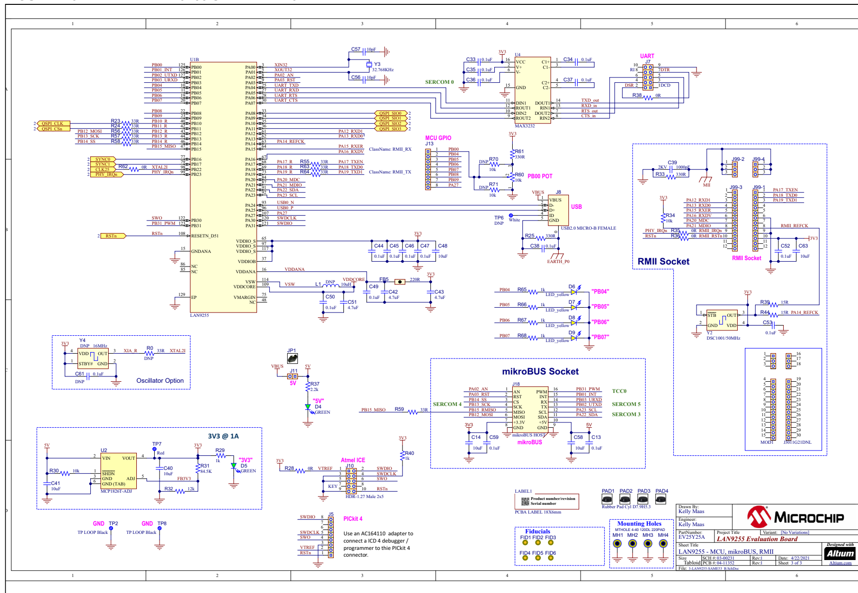
FIGURE A-3: EVB-LAN9255 SCHEMATIC 3
