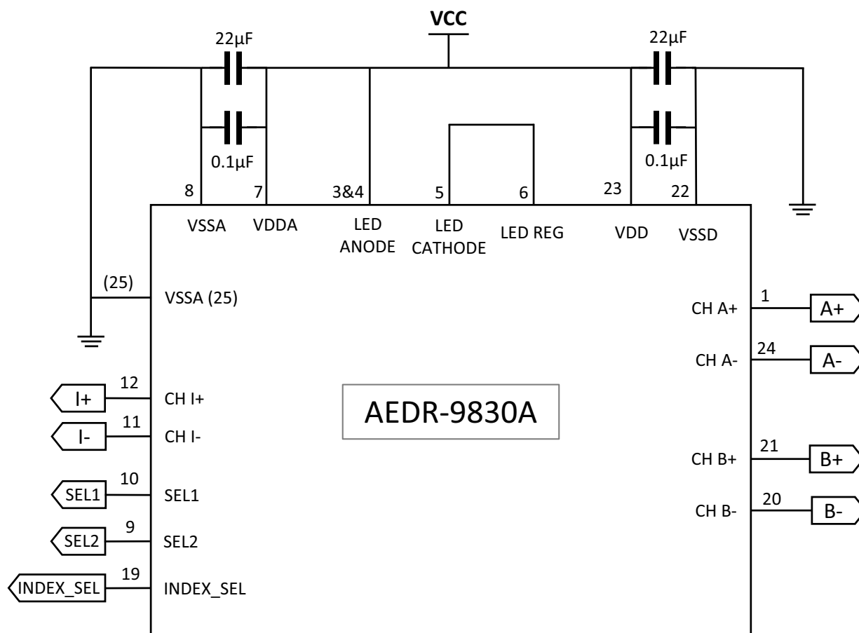
Figure 5: Reference Schematic Diagram for AEDR-9830A
