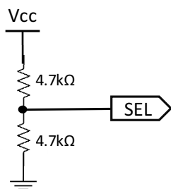
Figure 4: Example of Voltage Divider Circuit
