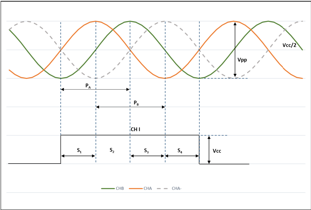
Figure 1: Analog Output Option
