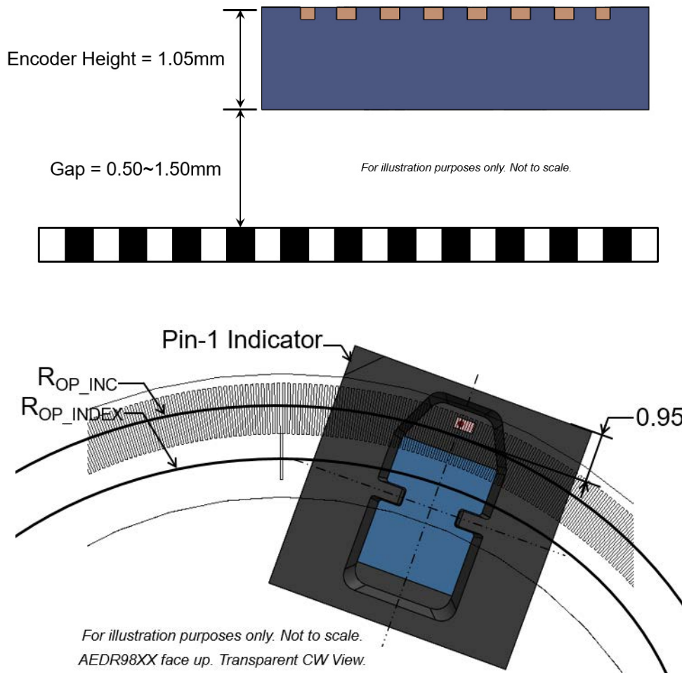
Figure 8: Encoder Placement Orientation
