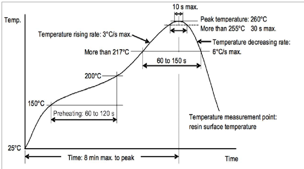
Figure 10: Typical Lead-Free Solder Reflow Soldering Temperature Profile
