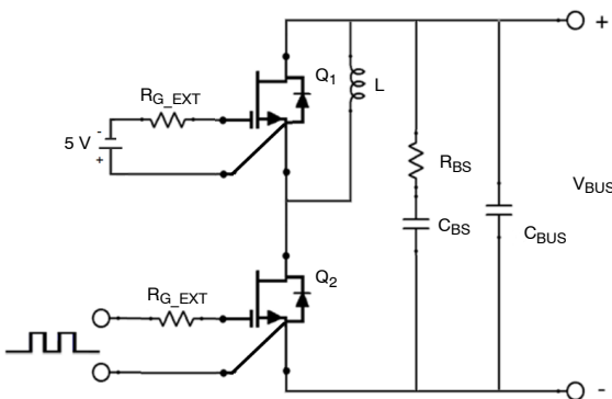
Figure 23. Schematic of the Half-bridge Mode Switching Test Circuit. Note, a Bus RC Snubber ( R_{BS} = 2.5 Ω, C_{BS} = 200 nF) Must be Applied to Reduce the Power Loop High Frequency Oscillations
