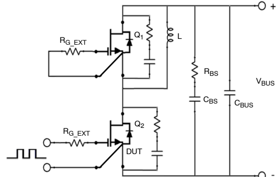
Figure 24. Schematic of the Half-bridge Mode Switching Test Circuit with Device RC Snubbers ( R_S = 5 Ω, C_S = 440 pF) and a Bus RC Snubber ( R_{BS} = 2.5 Ω, C_{BS} = 200 nF)
