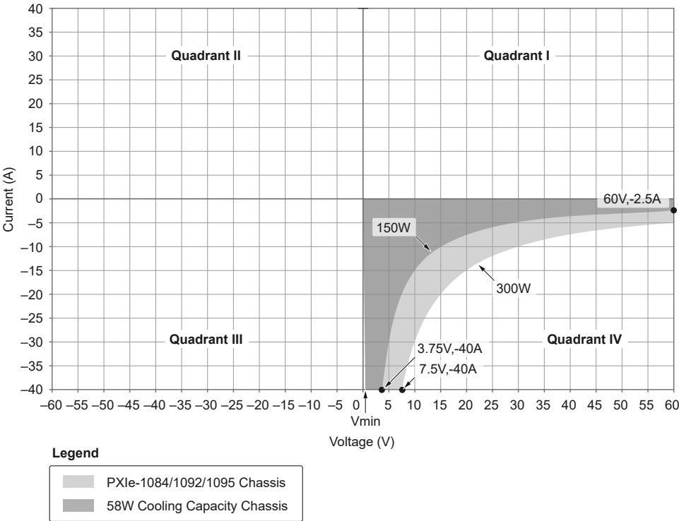
Figure 1. PXle-4051 Quadrant Diagram
