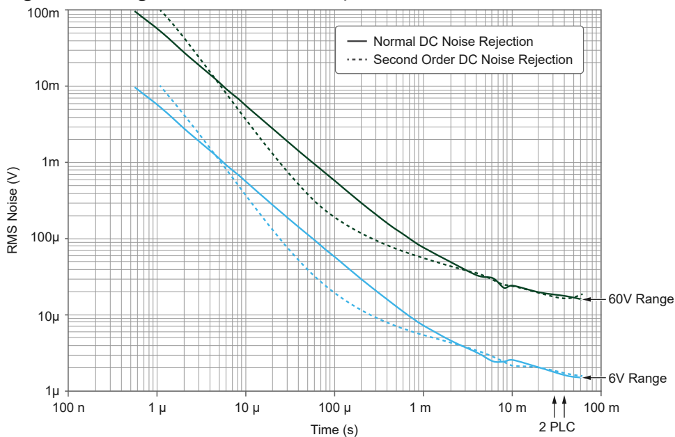
Figure 3. Voltage RMS Noise Versus Aperture Time, Nominal
