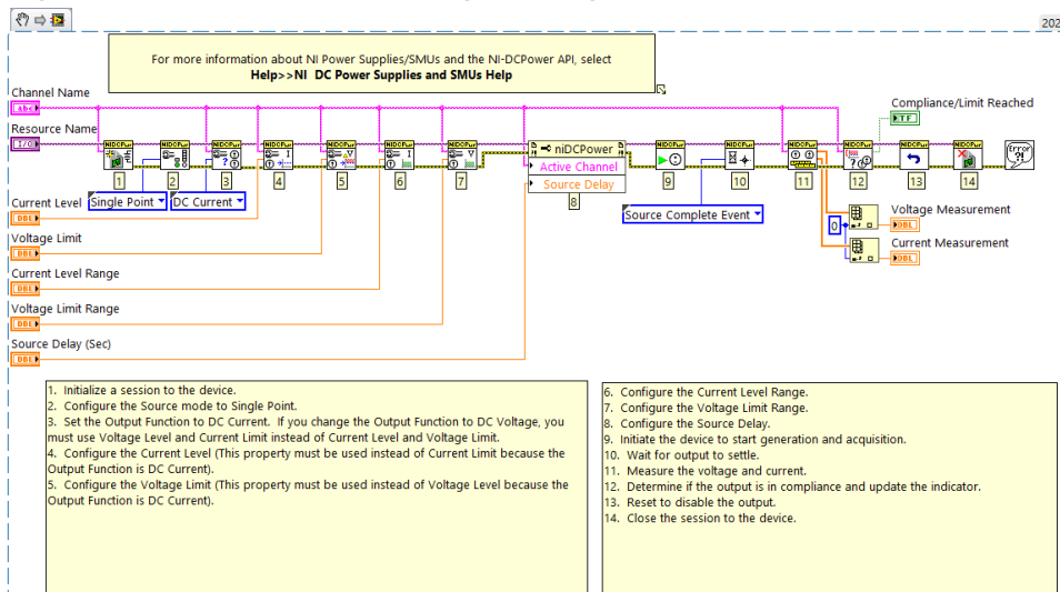
Figure 11. NI-DCPower Sourcing/Sinking Current Example
