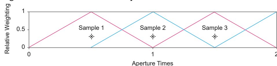
Figure 23. Second-Order Noise Rejection
