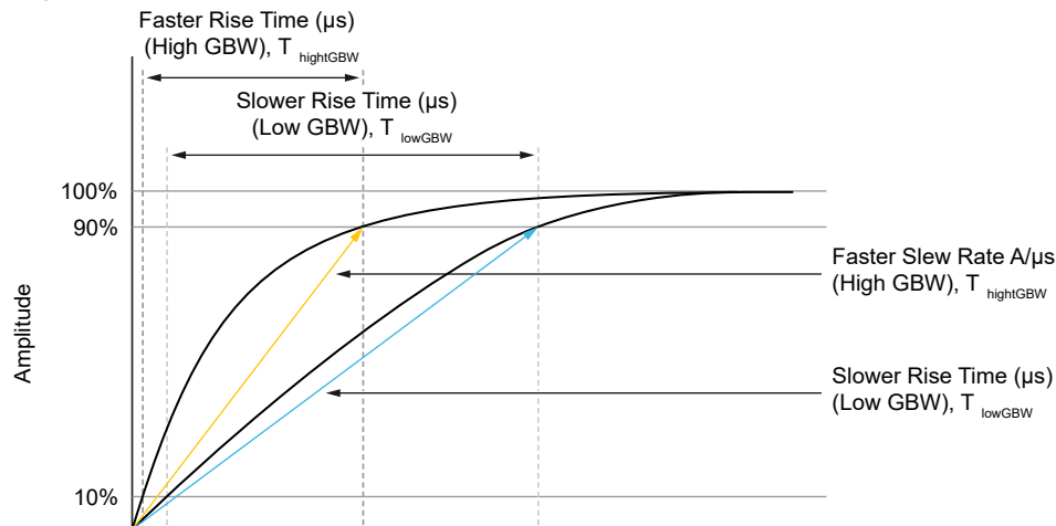
Figure 17. Limitations on Slew Rates based on GBW
