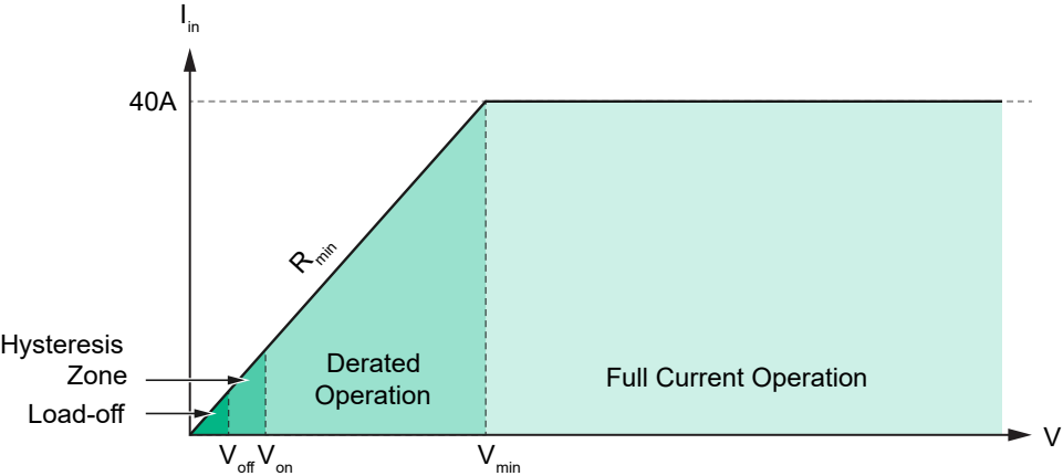
Figure 19. Zones of Operation
