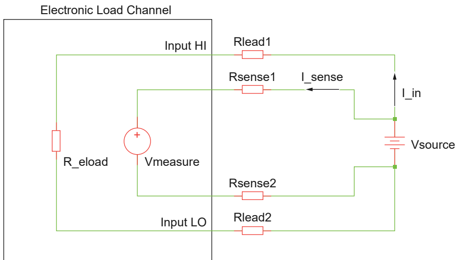
Figure 8. Connecting for a Remote Sense Measurement
