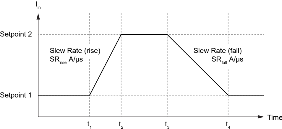
Figure 16. Programmable Slew Rates in Constant Current Mode
