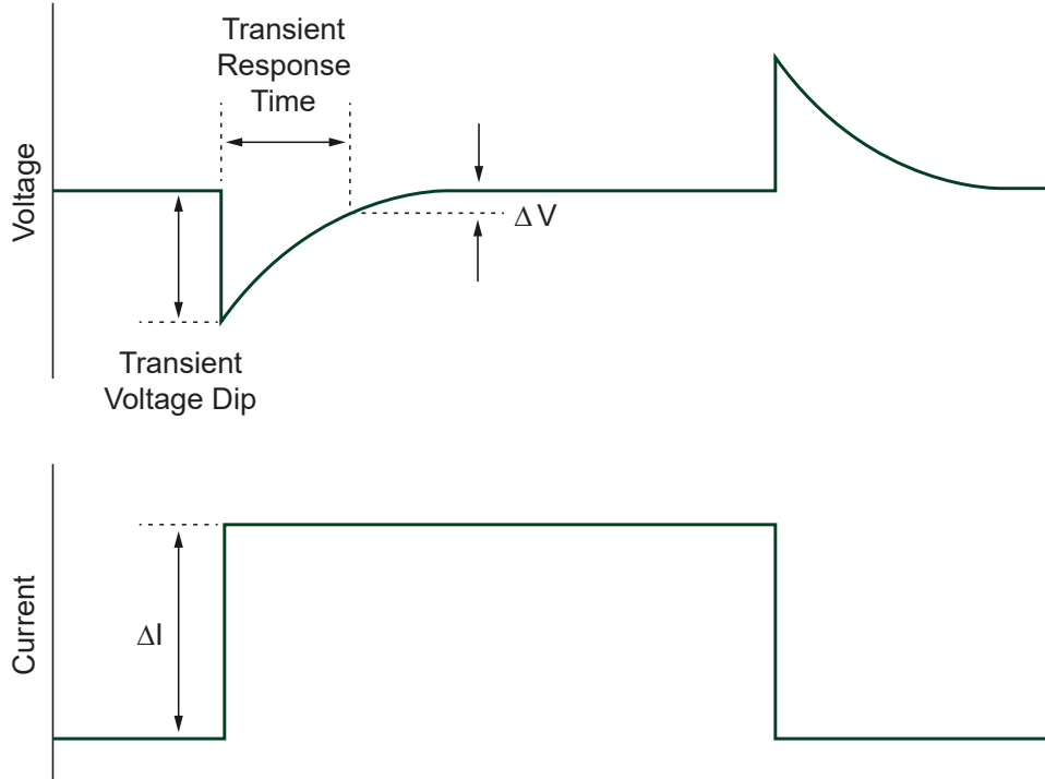
Figure 15. Transient Response
