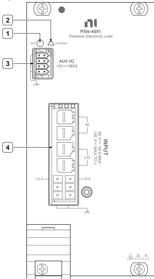
Figure 3. PXIe-4051 Front Panel
