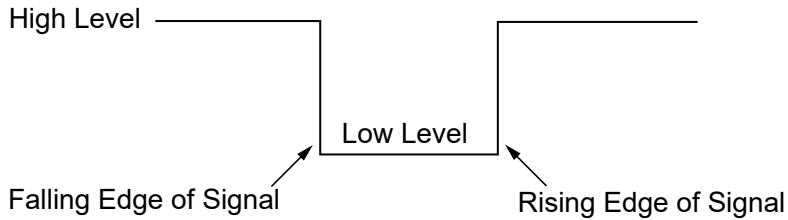
Figure 14. Digital Edge Trigger
