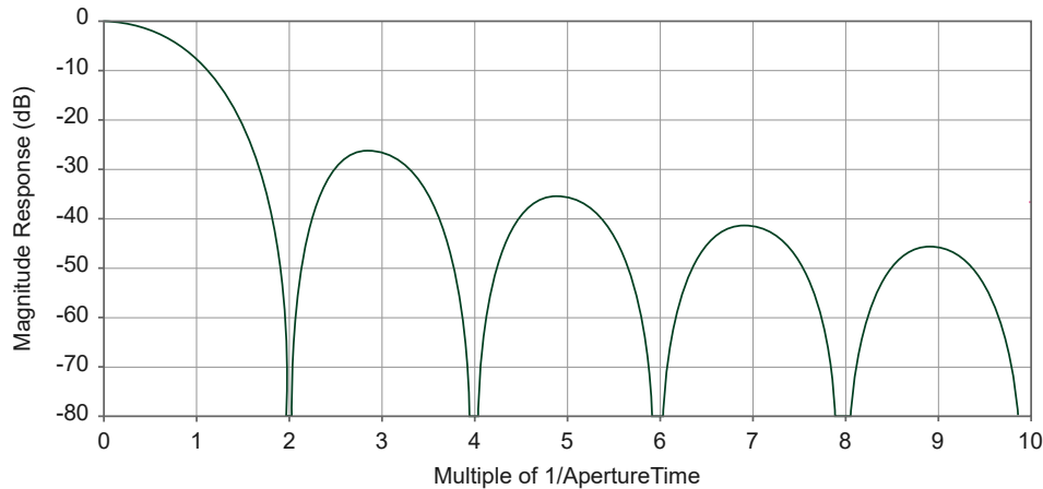
Figure 24. Second-Order Noise Rejection by Frequency
