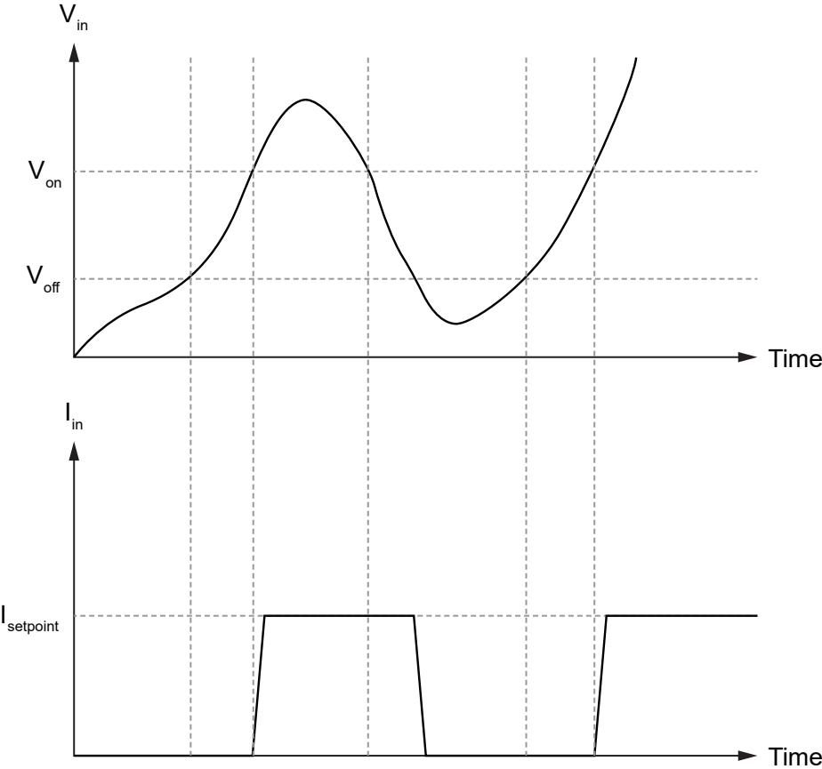
Figure 20. V_{on} and V_{off} Behaviors
