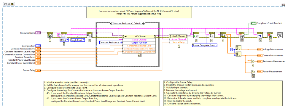
Figure 13. NI-DCPower Constant Resistance and Constant Power Example
