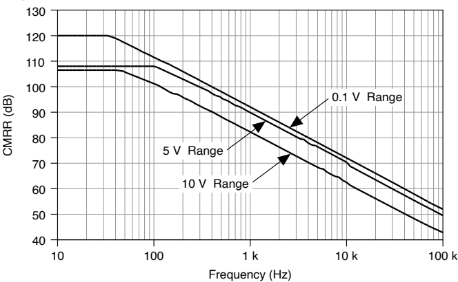
Figure 2. CMRR
