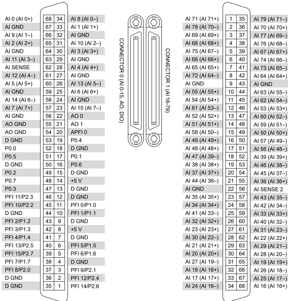
Figure 1. NI PXIe-6355 Pinout
