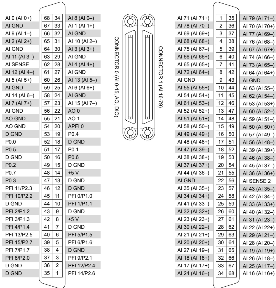
Figure 2. NI PXle-6365 Connector 0 and 1 Pinout
