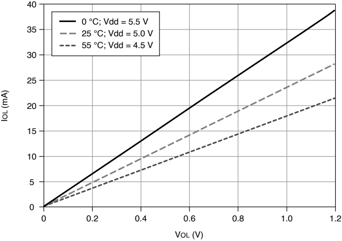
Figure 12. PFI <0..15>/P1/P2: I_{OL} versus V_{OL}
