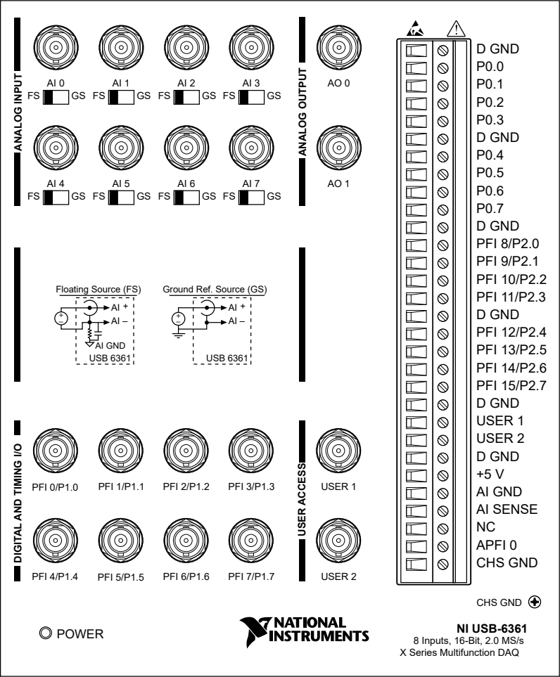
Figure 4. NI USB-6361 BNC Front Panel and Pinout
