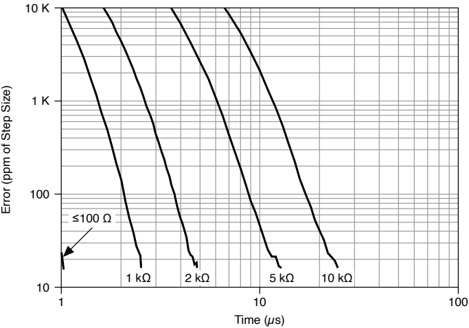
Figure 5. Settling Error versus Time for Different Source Impedances
