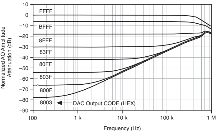
Figure 8. AO External Reference Bandwidth
