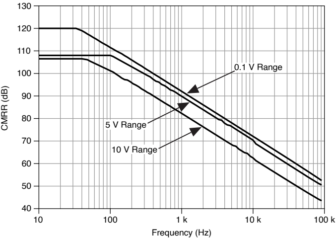
Figure 7. AI <0..15> CMRR
