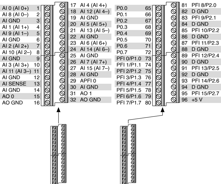
Figure 3. NI USB-6361 Screw Terminal Pinout
