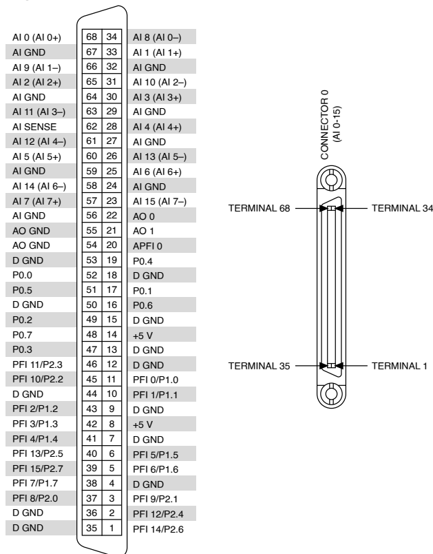
Figure 1. NI PCIe/PXIe-6361 Pinout
