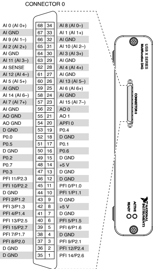
Figure 3. NI USB-6361 Screw Terminal Pinout
