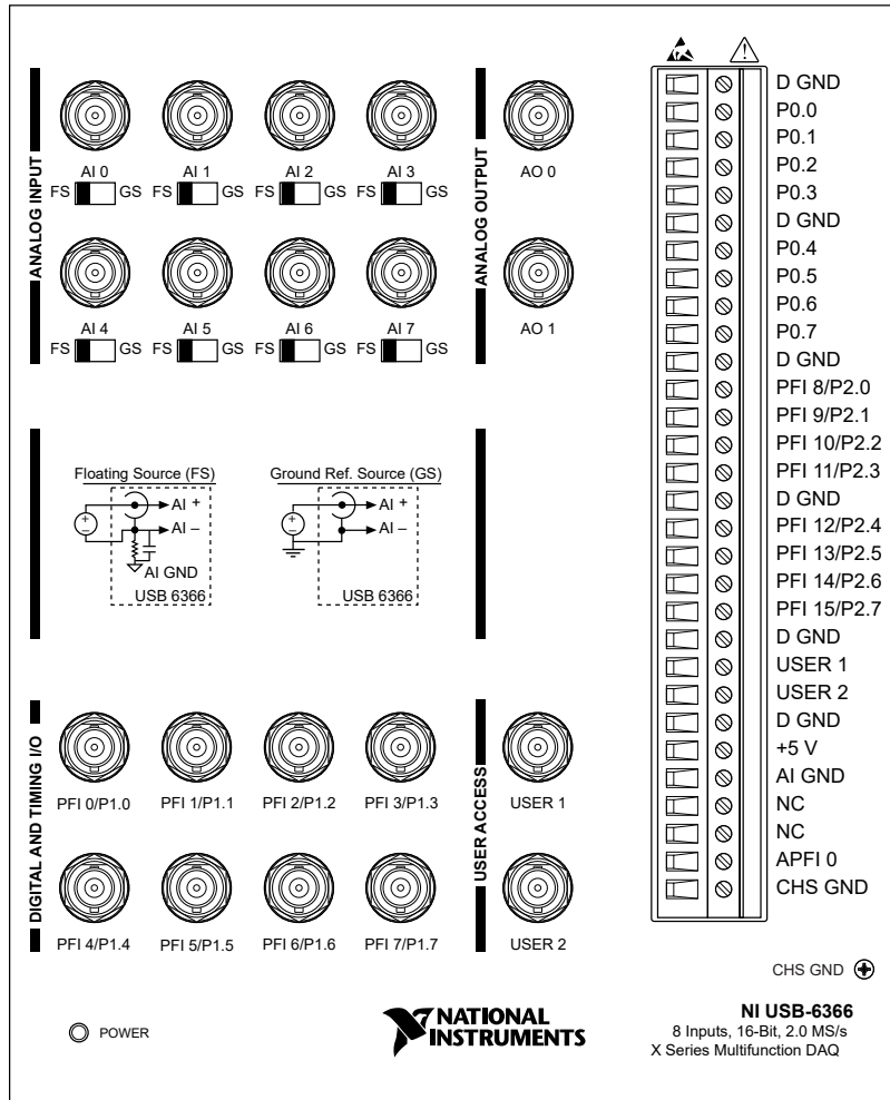
Figure 4. NI USB-6366 BNC Front Panel and Pinout
