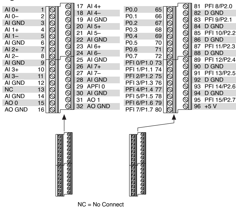
Figure 3. NI USB-6366 Screw Terminal Pinout
