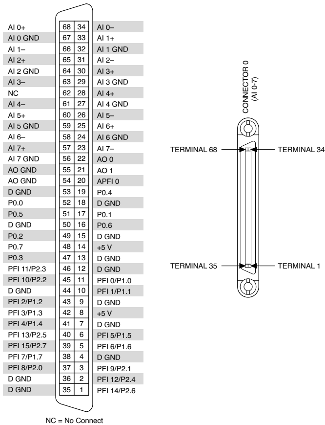
Figure 1. NI PXIe-6366 Pinout
