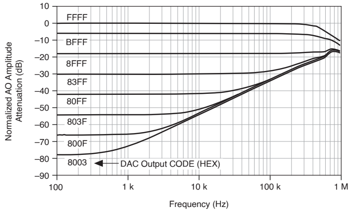
Figure 5. Analog Output External Reference Bandwidth
