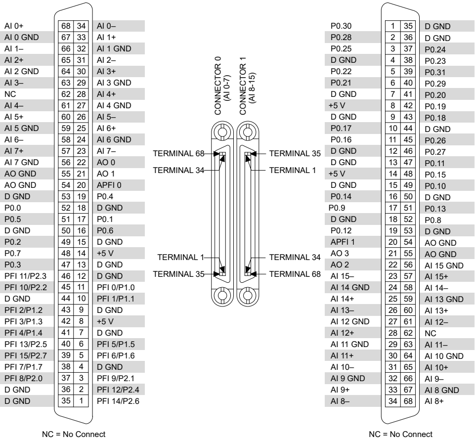
Figure 1. NI PXIe-6368 Pinout
