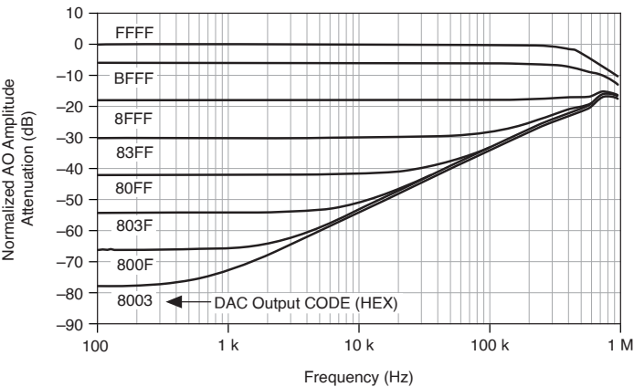
Figure 2. Analog Output External Reference Bandwidth
