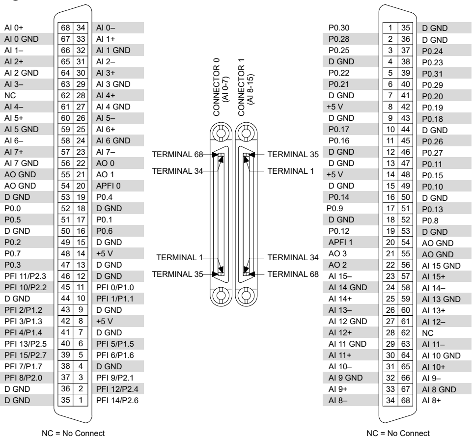
Figure 1. NI PXIe-6358 Pinout
