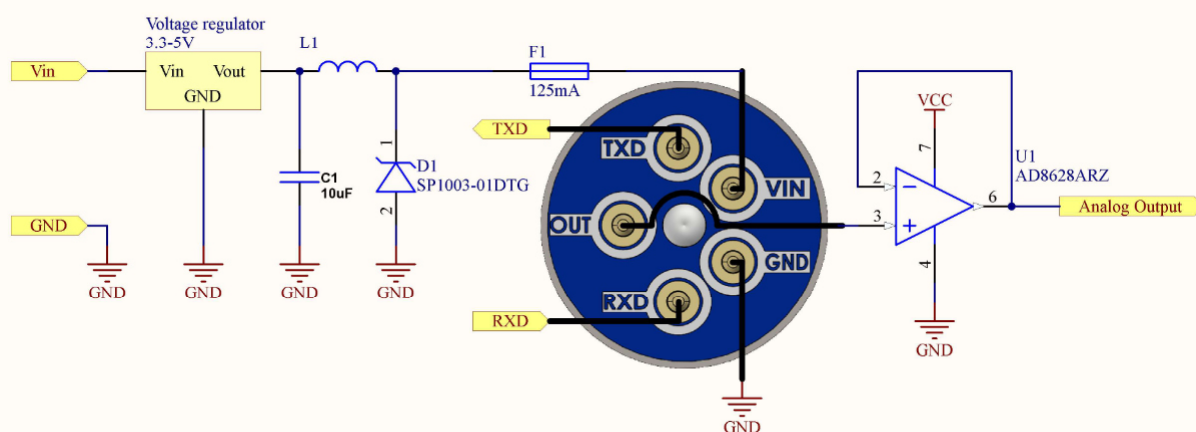
Fig.1 Example schematic for Interfacing Integrated IR (INIR2-CD100)
