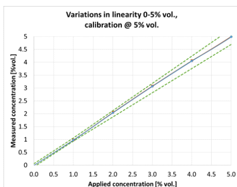
Typical Linearity 0-5%
