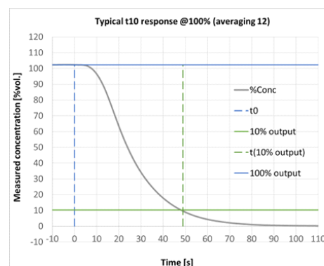
Typical recovery time @100%
