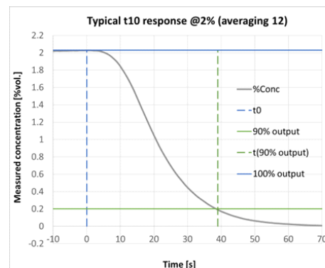
Typical recovery time @2%
