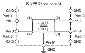
Equivalent Circuit
