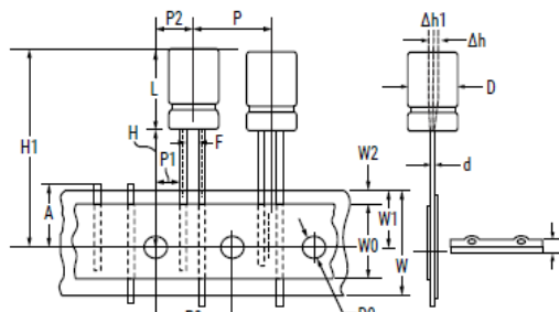
Fig. 4 (Diameter for \Phi 10 ) 10 mm EA
