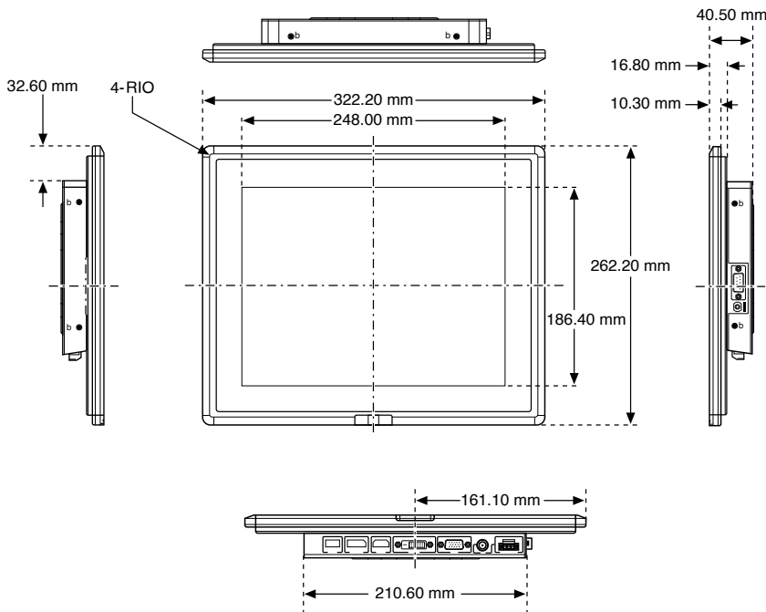
Figure 5. NI TSM-1015 Dimensions
