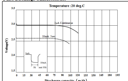
Pulse Discharge Characteristics
