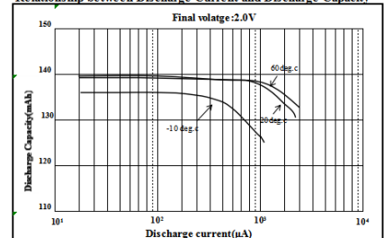
Relationship between Discharge Current and Discharge Capacity
