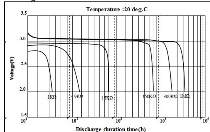
Discharge Characteristics
