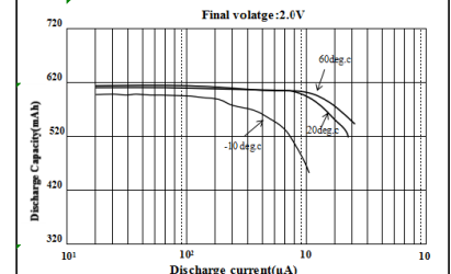
Relationship between Discharge Current and Discharge Capacity
