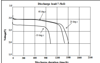
Discharge Characteristics
