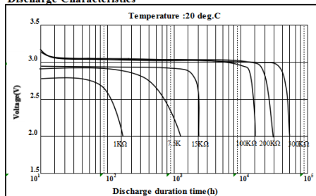
Discharge Characteristics
