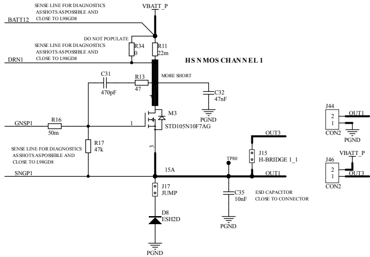
Figure 12. EVL-L98GD8 evaluation board schematics (part 2/3)
