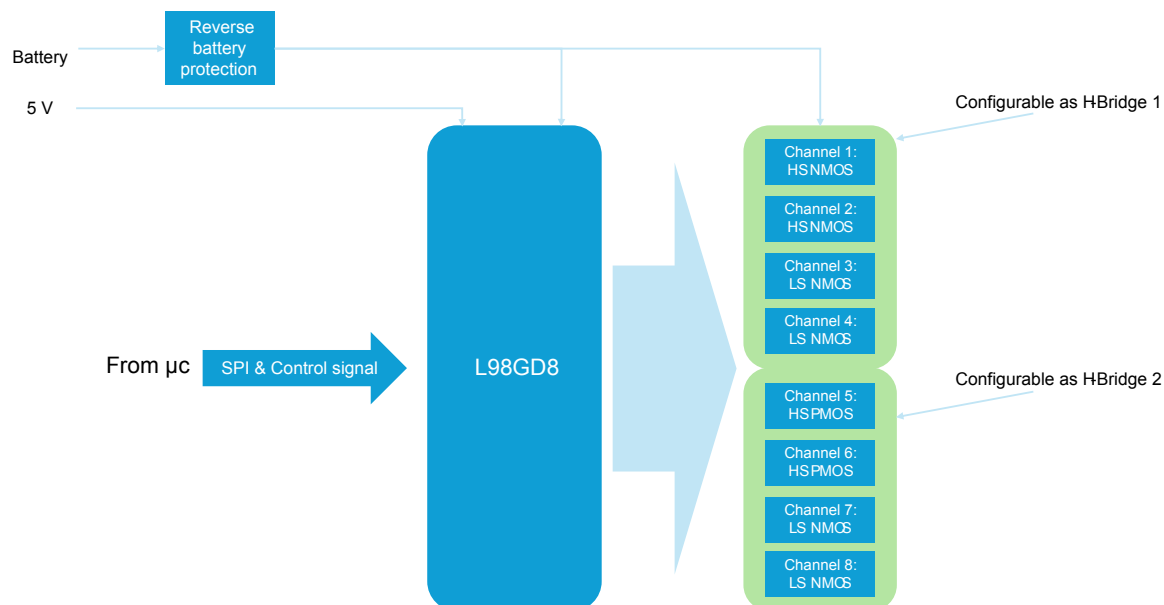
Figure 14. EVL-L98GD8 evaluation board configuration block diagram
