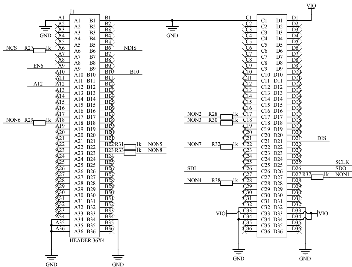
Figure 10. Microcontroller connectors
