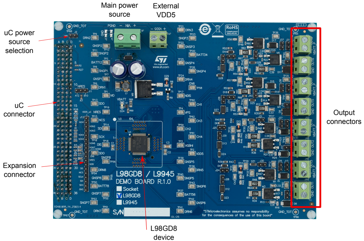
Figure 9. Motherboard main components and connectors
