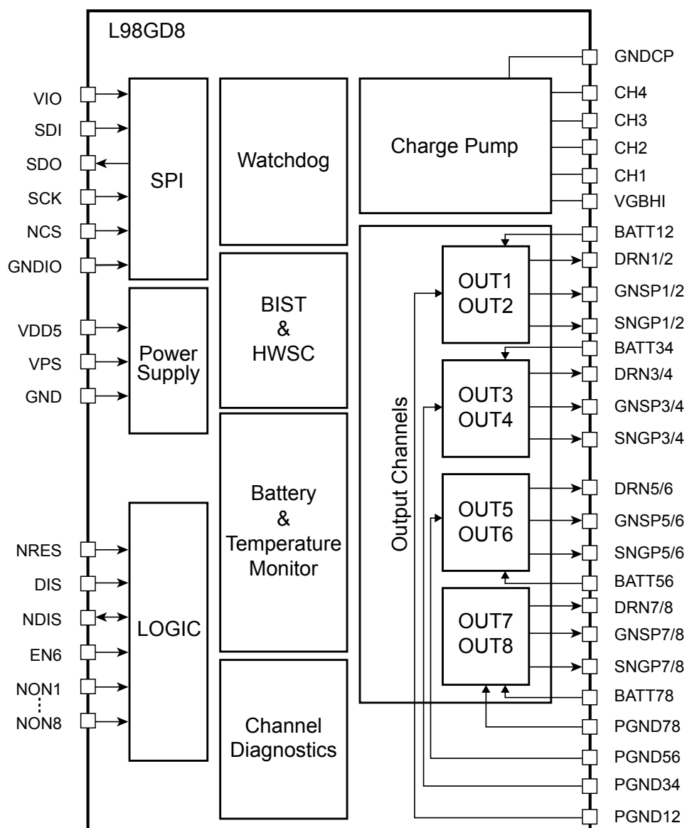
Figure 2. L98GD8 block diagram
