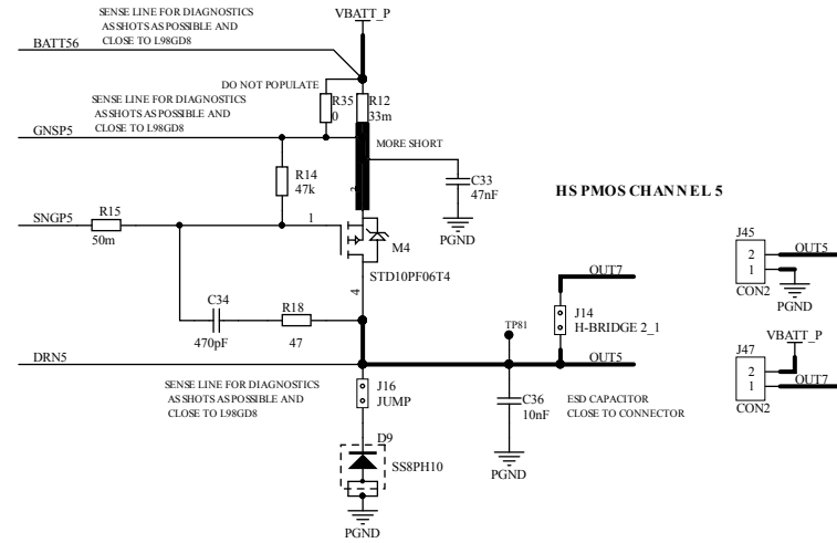
Figure 12. EVL-L98GD8 evaluation board schematics (part 2/3)
