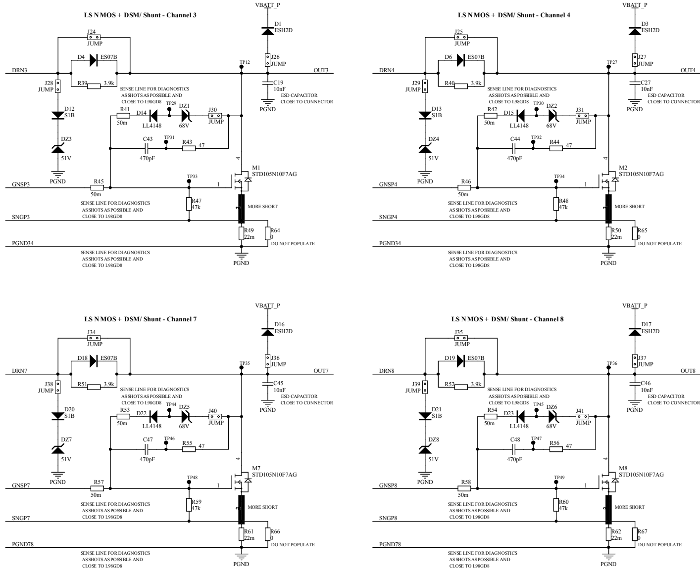
Figure 13. EVL-L98GD8 evaluation board schematics (part 3/3)
