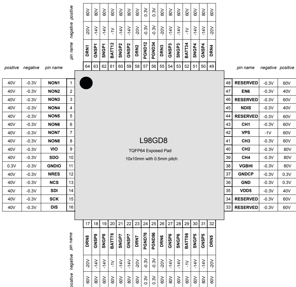
Figure 3. L98GD8 pinout
