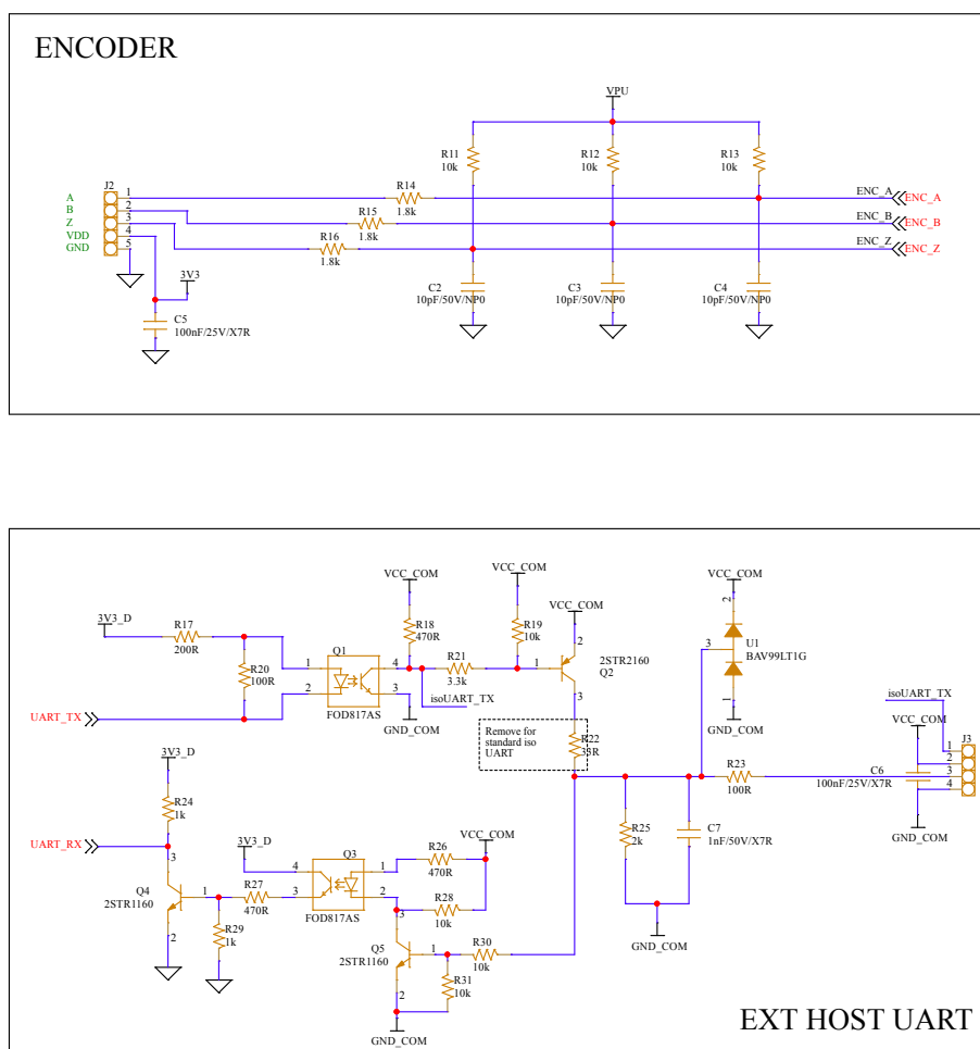
Figure 3. EVSTDRVG611MC schematic - peripherals
