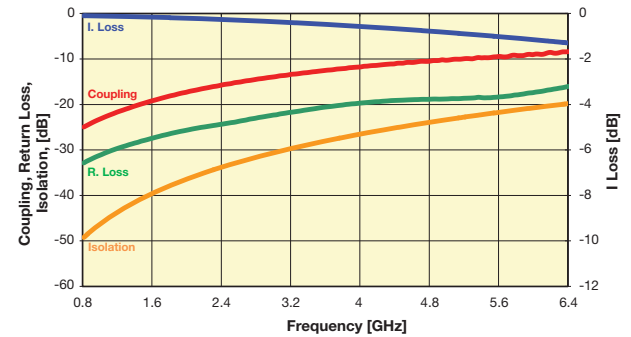
CP0603AxxxxMNTR
