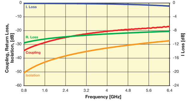
CP0603AxxxxGNTR
