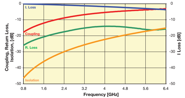
CP0603AxxxxHNTR
