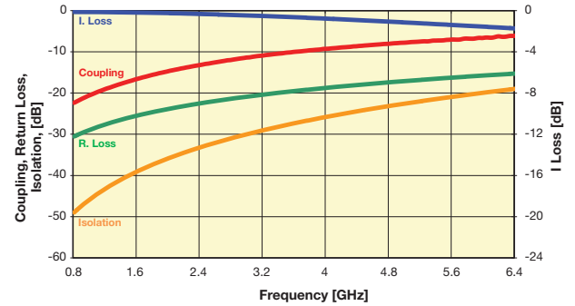
CP0603AxxxxDNTR
