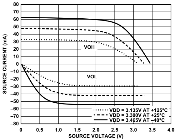
Figure 36. Driver Type A Current for All Pins Operating Above 62.5 MHz and Less Than or Equal to 166.66 MHz (3.3 V V_{DD\_EXT} )
