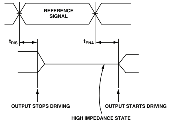
Figure 38. Output Enable/Disable
