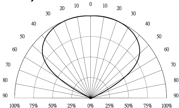
Radiation Diagram
