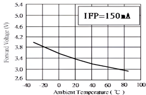
Forward Voltage vs. Ambient Temperature
