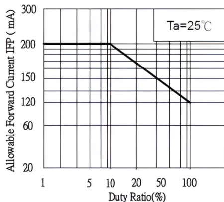
Duty Ratio vs. Allowable Forward Current
