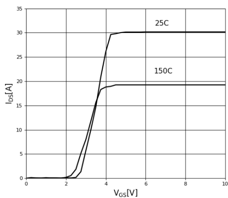
Figure 6. Typical Transfer Characteristics V_{DS} = 10\text{V} , parameter: T_J
