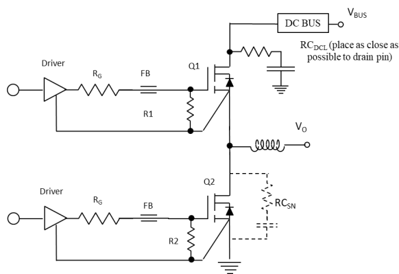
Figure 2. Simplified Half-bridge Schematic
