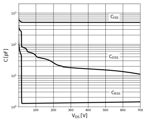
Figure 8. Typical Capacitance V_{GS} = 0\text{V} , f = 1\text{MHz}
