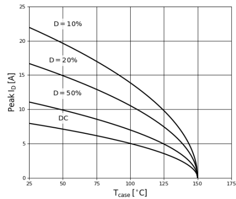
Figure 13. Current Derating
