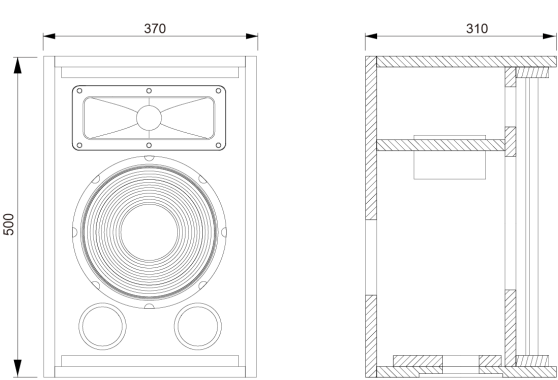
Speaker Drawing
