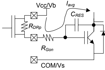
Figure 20: R_{Gon} Sizing
