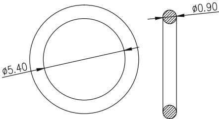
O-ring (P/N: OR-150)
