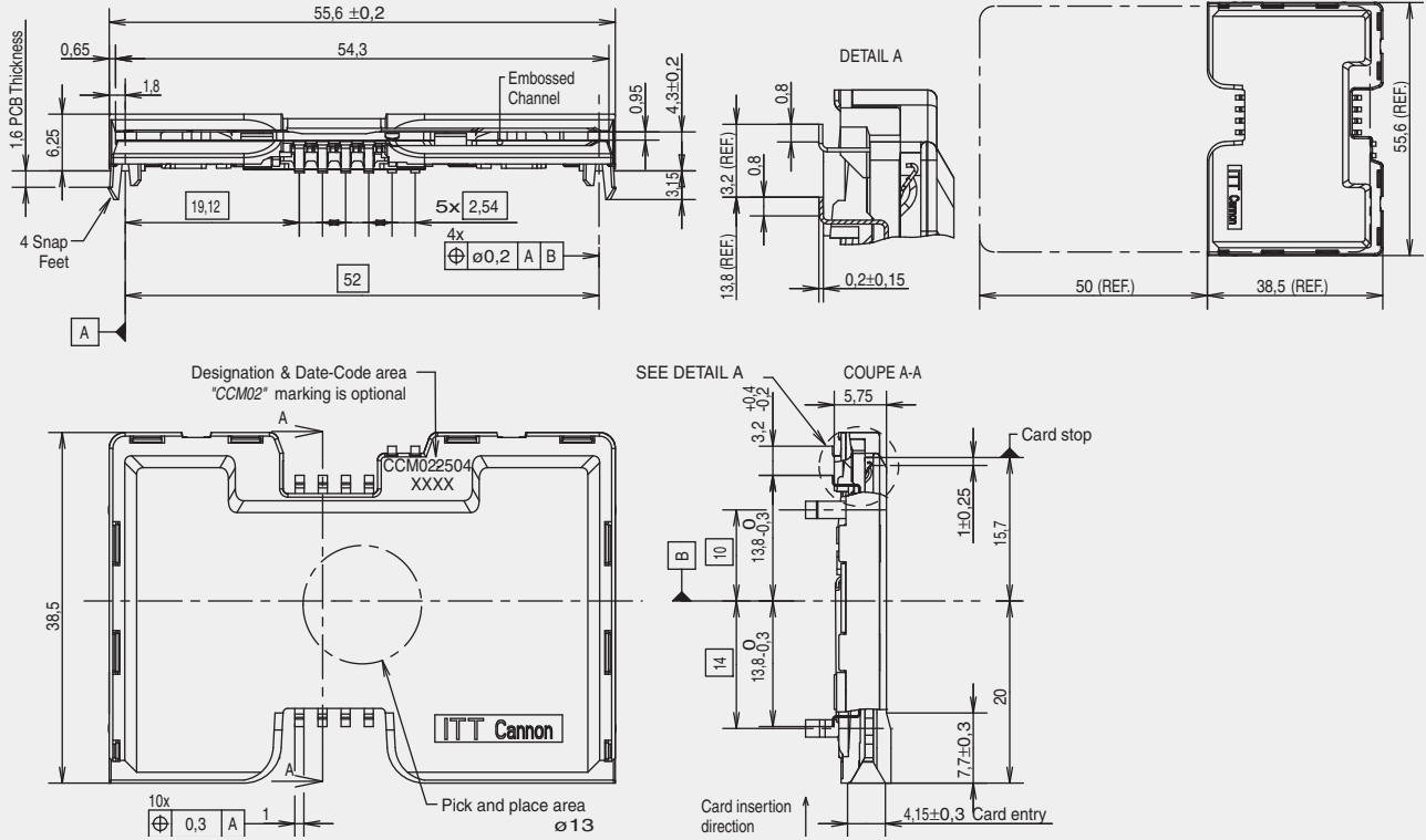
CCM02-2504 (8 contacts SMT - 4 board lock)
