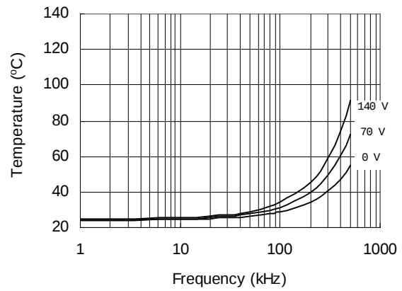
Figure 28. IRS21834 vs. Frequency (IRFBC40), R_{gate}=15 \Omega , V_{CC}=15 \text{ V}
