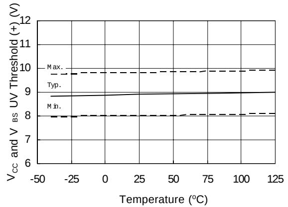
Figure 18. V_{CC} and V_{BS} Undervoltage Threshold (+) vs. Temperature
