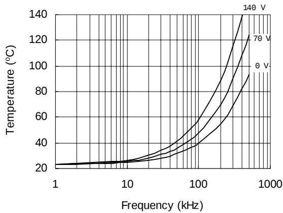
Figure 29. IRS21834 vs. Frequency (IRFPE50), R_{gate}=10 \Omega , V_{CC}=15 \text{ V}
