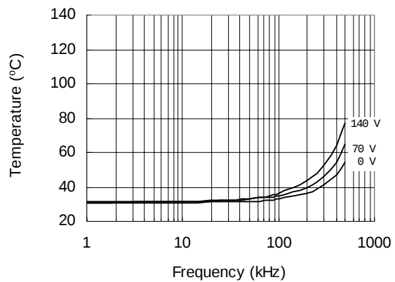
Figure 30. IRS2183S vs. Frequency (IRFBC20), R_{gate}=33 \Omega , V_{CC}=15 \text{ V}
