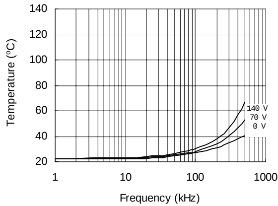
Figure 27. IRS21834 vs. Frequency (IRFBC30), R_{gate}=22 \Omega , V_{CC}=15 \text{ V}
