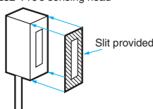
E32-T16's sensing head
