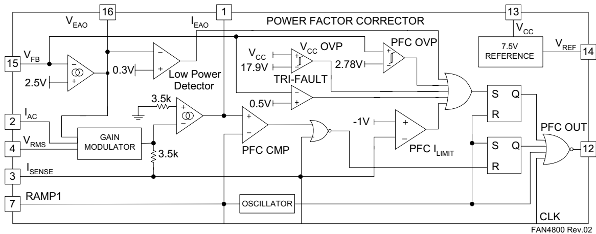
Figure 7. PFC Section Block Diagram
