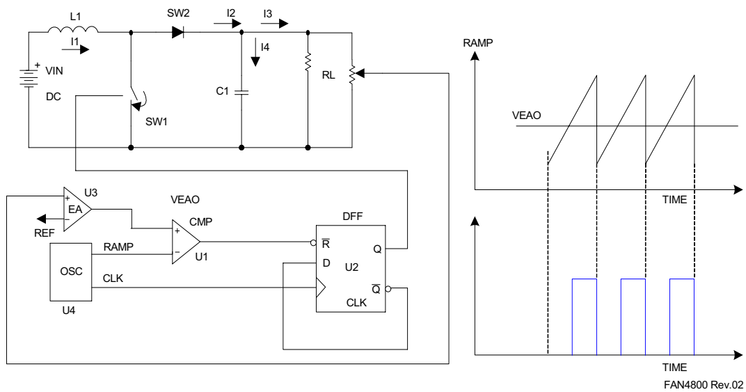
Figure 11. Typical Leading-Edge Control Scheme
