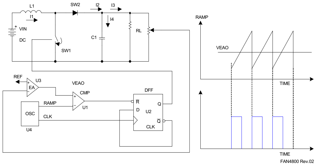
Figure 10. Typical Trailing-Edge Control Scheme
