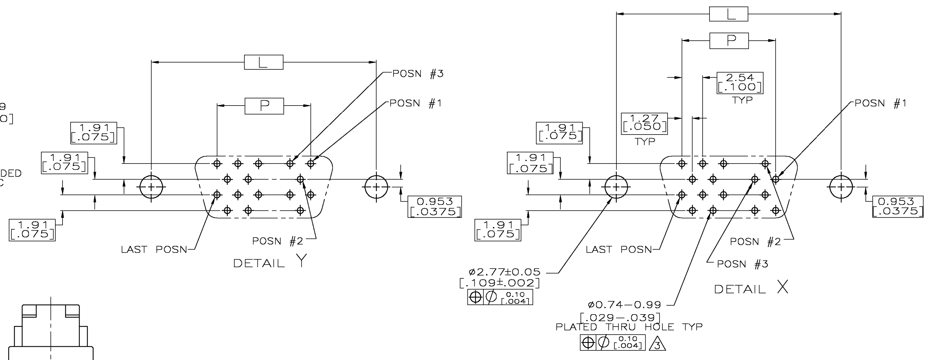
P.C. BOARD MOUNTING DIMENSIONS (CONNECTOR SIDE)
