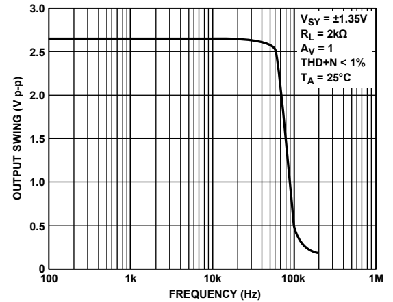
Figure 36. Maximum Output Swing vs. Frequency at 2.7 V
