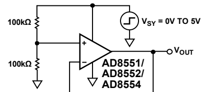
Figure 64. AD855x Test Circuit for Turn-On Time
