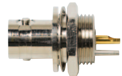
BNC (F) Bulkhead Receptacle, Isolated Ground, PTFE, 75Ω 6741
