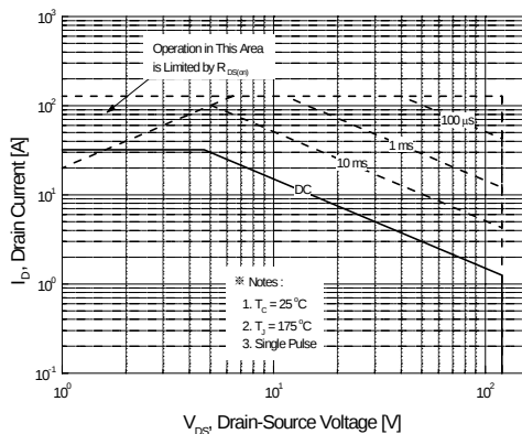
Figure 9-1. Maximum Safe Operating Area for FQP32N12V2
