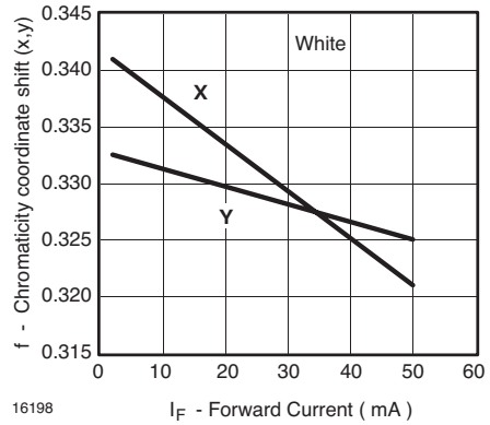
Figure 46. Chromaticity Coordinate Shift vs. Forward Current
