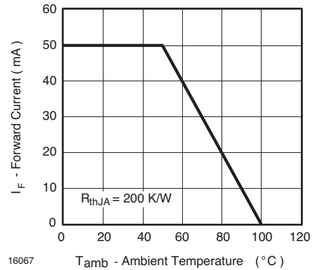
Figure 4. Forward Current vs. Ambient Temperature for InGaN
