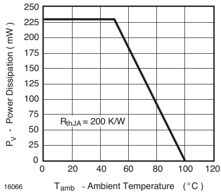
Figure 1. Power Dissipation vs. Ambient Temperature for InGaN
