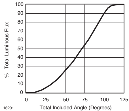
Figure 4. Percentage Total Luminous Flux vs. Total Included Angle for 90\text{ }^{\circ} emission angle
