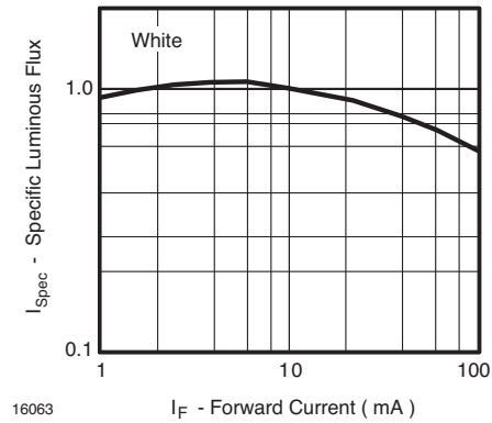
Figure 8. Specific Luminous Flux vs. Forward Current
