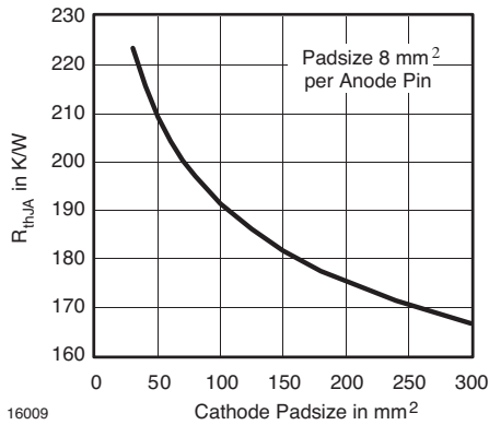
Figure 5. Thermal Resistance Junction Ambient vs. Cathode Padsizes
