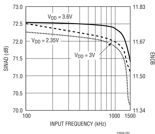
Figure 7. LTC2366 ENOB and SINAD vs Input Frequency
