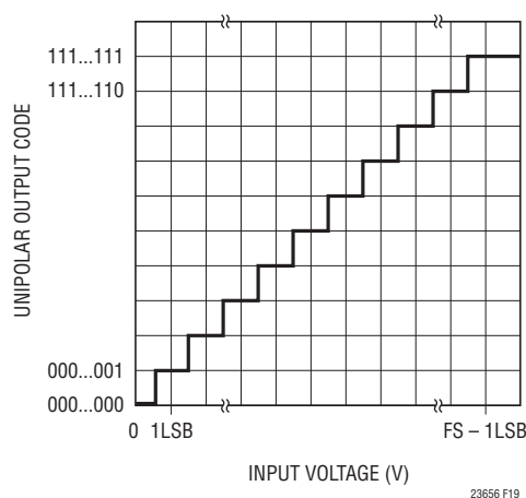
Figure 19. LTC2365/LTC2366 Transfer Characteristics
